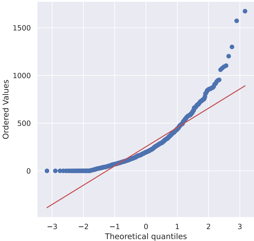
Rainfall — Q-Q Plot
