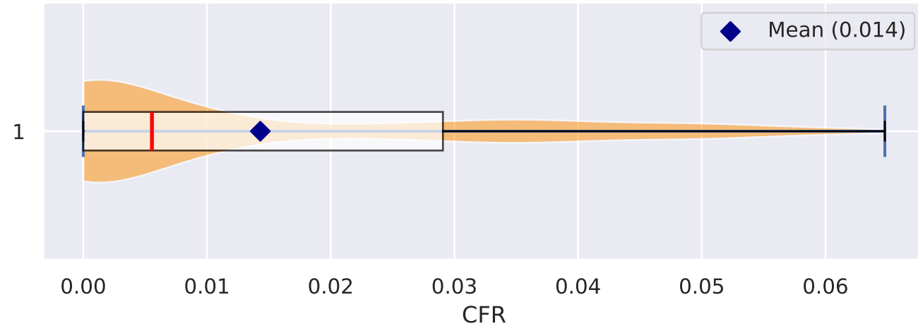
HFRS — Violin
