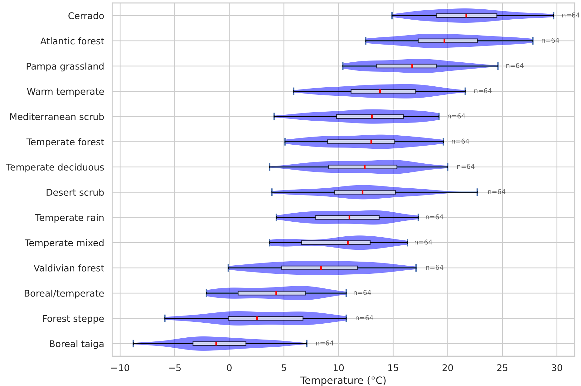
Temperature by Biome (sorted coldest → warmest)
