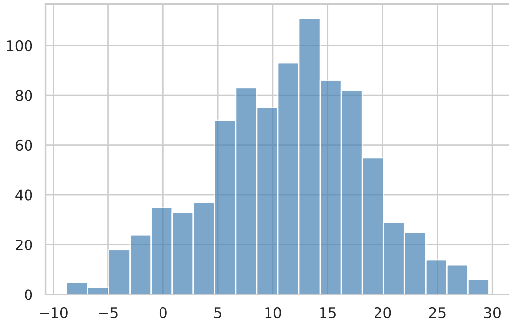
Histogram
