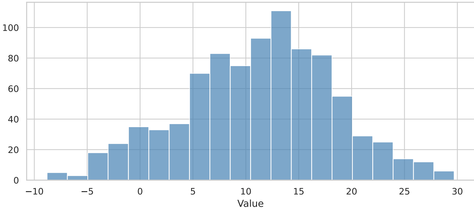
Average Temperature (°C) — Histogram (FD rule)
