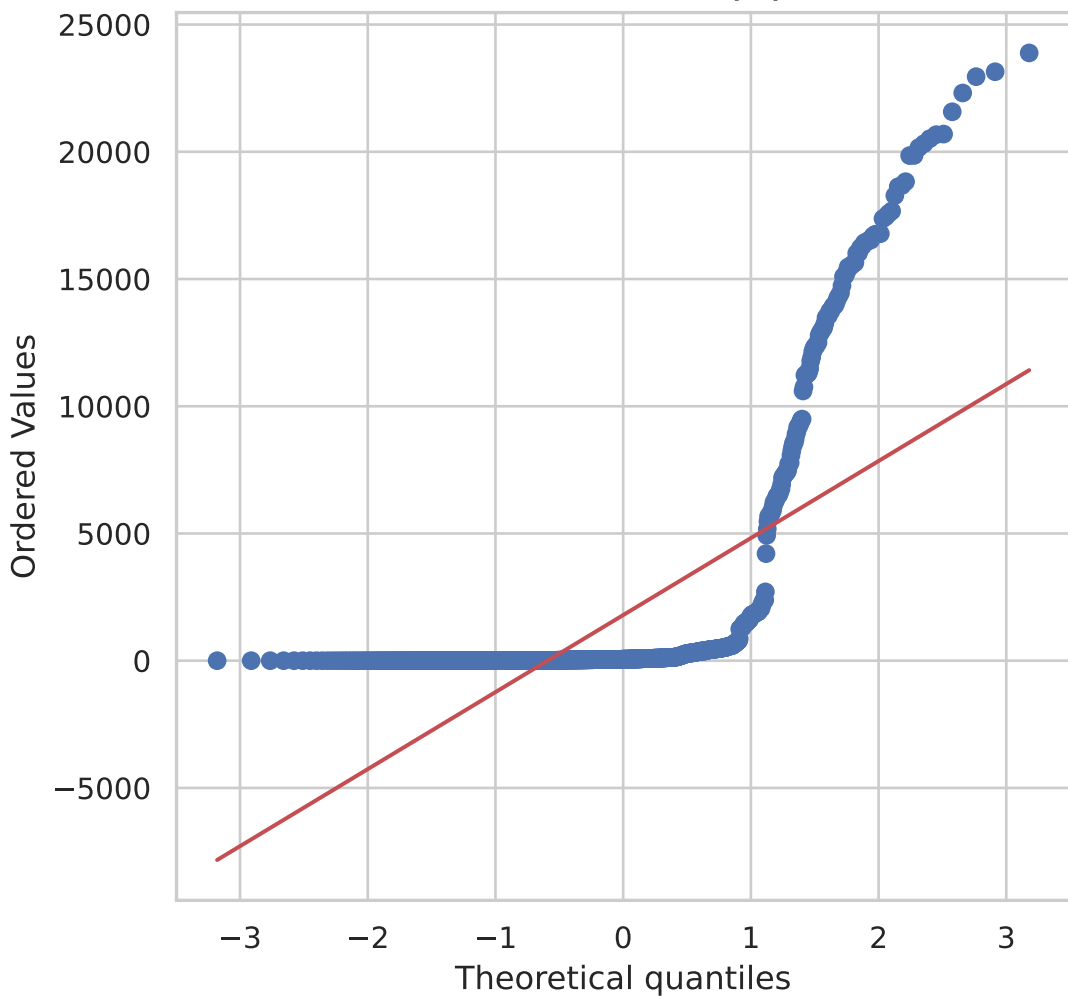
Confirmed Cases — Q-Q Plot
