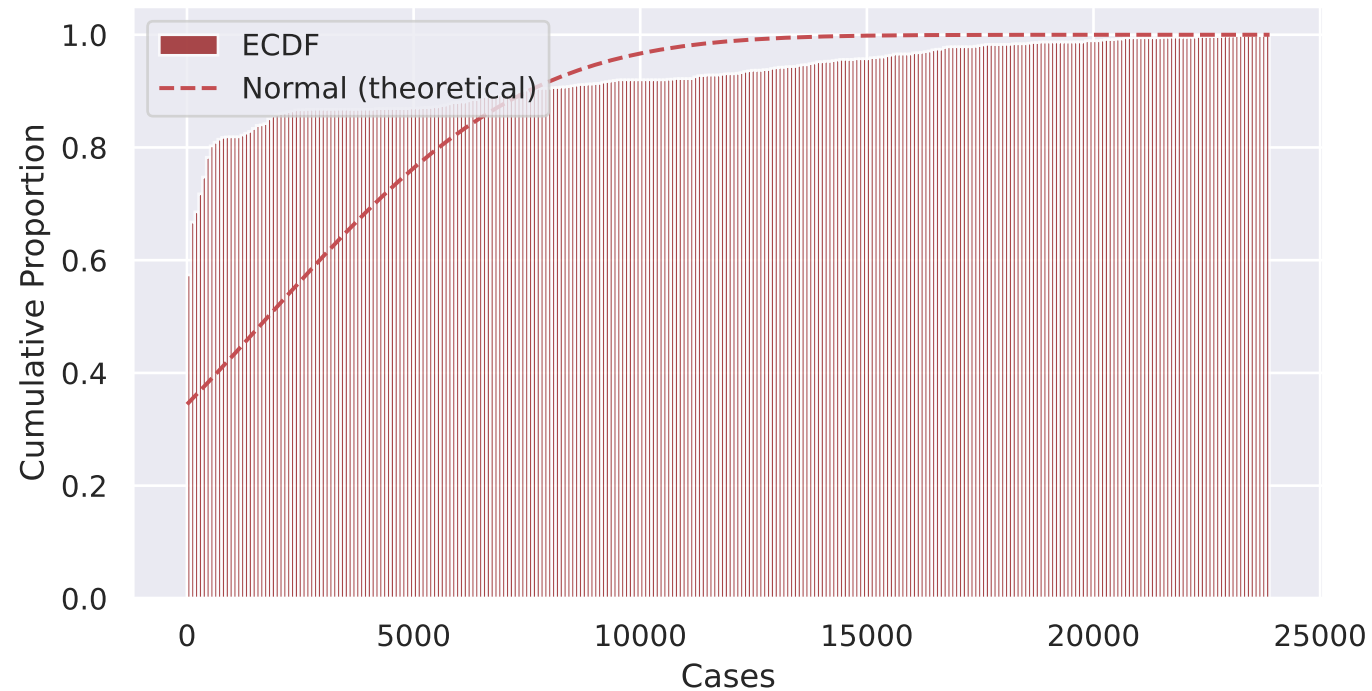
Confirmed Cases — All Data ECDF
