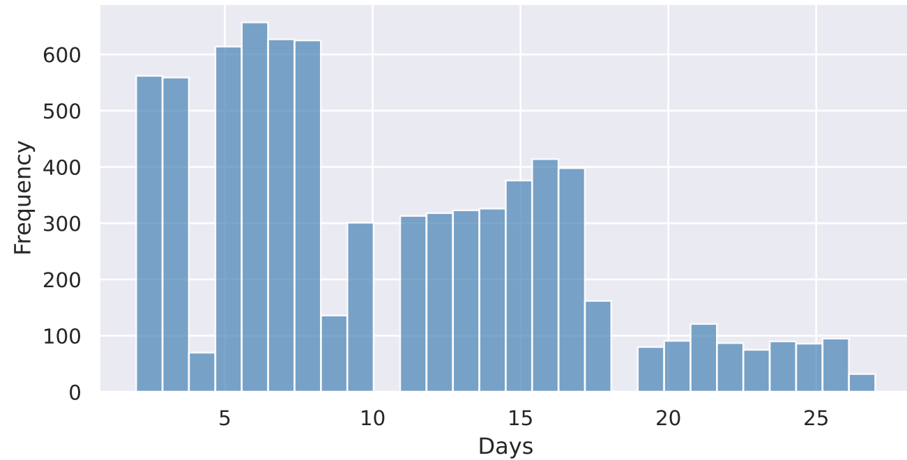
Hospital Days — Original Scale
