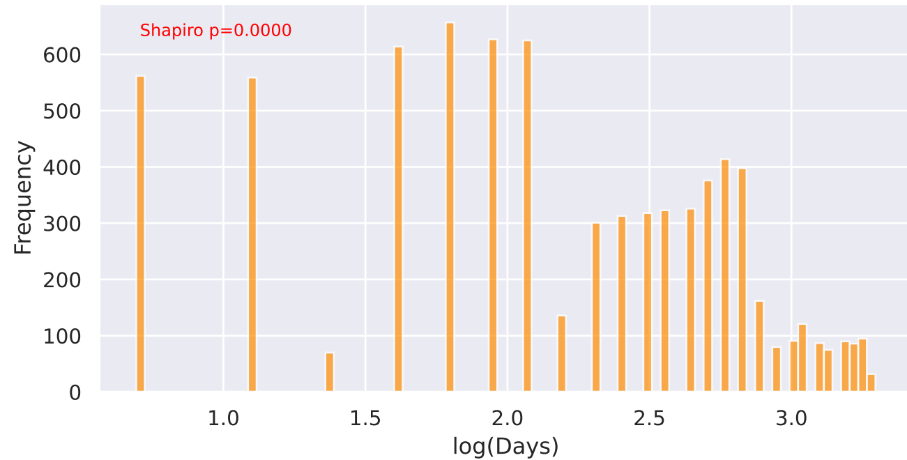
Hospital Days — Log-Transformed
