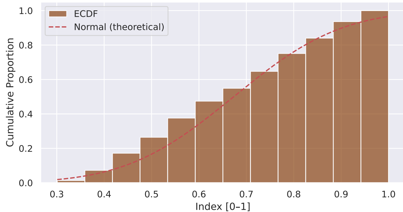
Rodent Abundance — Cumulative Normalized Histogram
