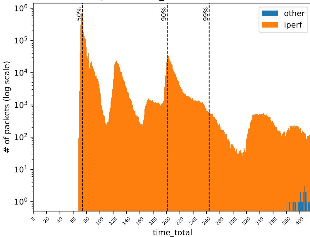
Histogram of time_total for XDP (GRO off)
