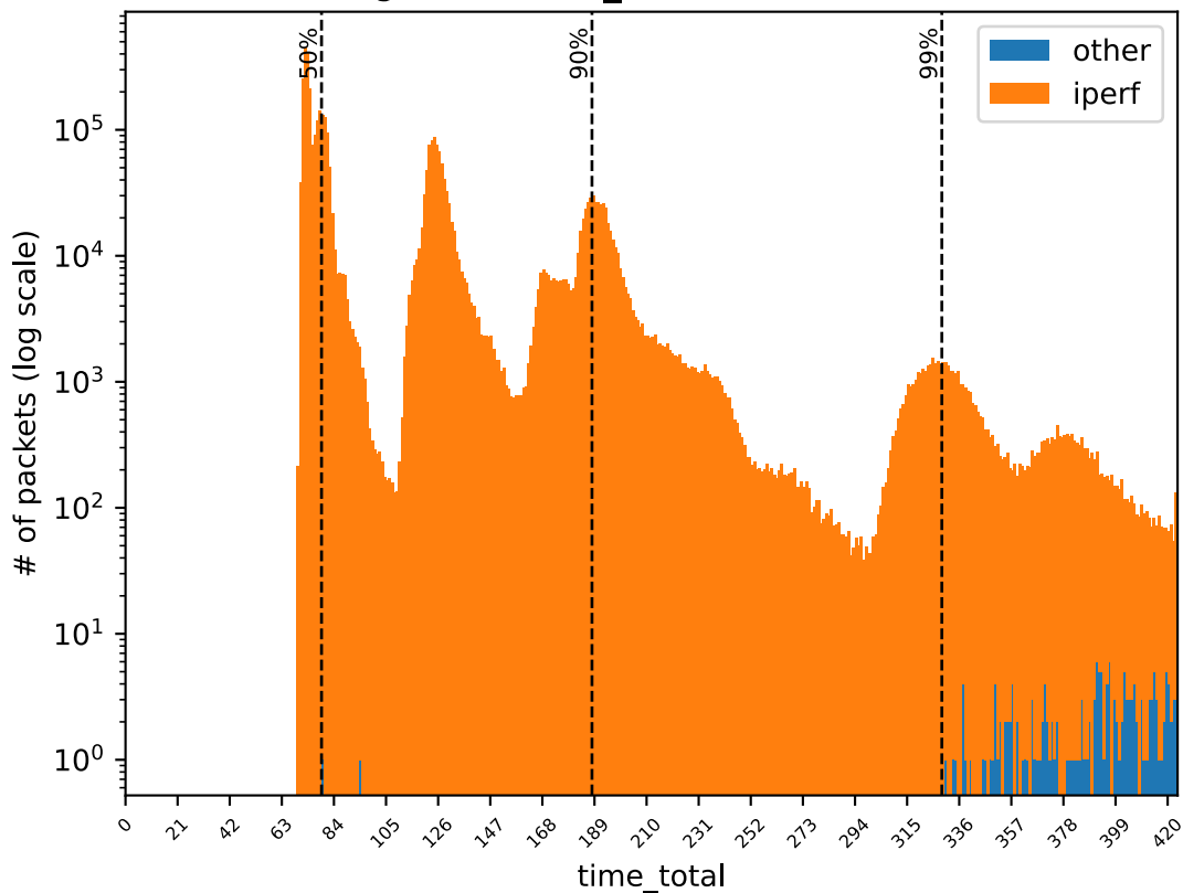
Histogram of time_total for XDP (GRO on)
