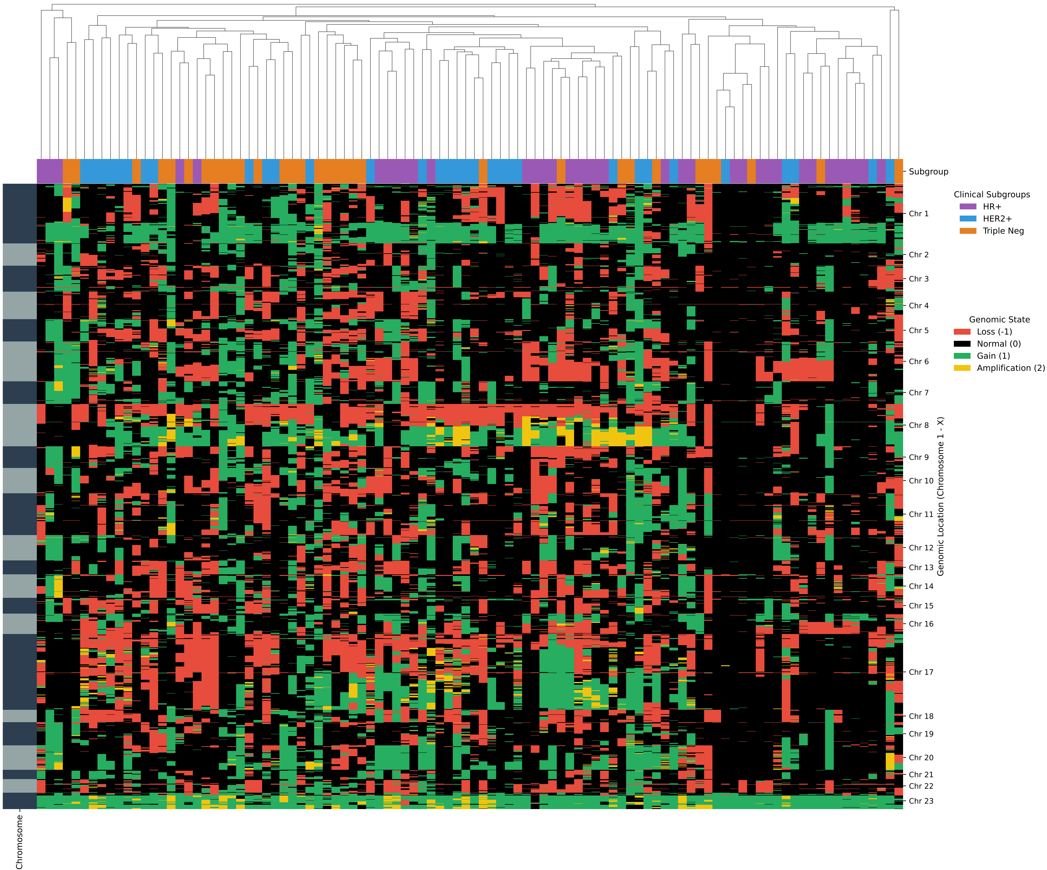
Genomic Portrait (Average Linkage + Pearson Correlation)
