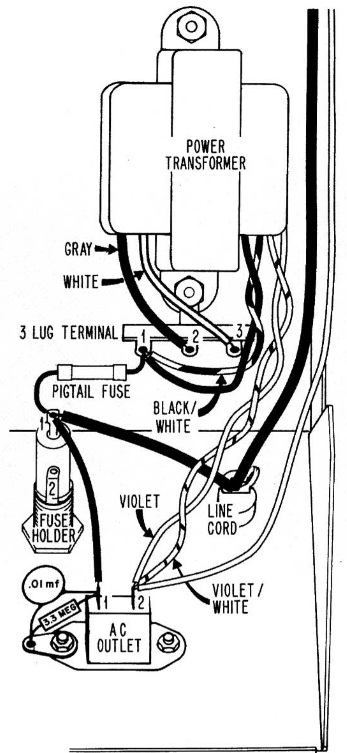
120 VOLT AC LINE WIRING FOR UNITS OBTAINED IN CANADA
