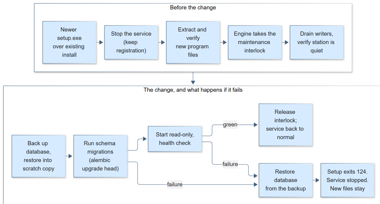
Figure 77: Upgrade and rollback.
