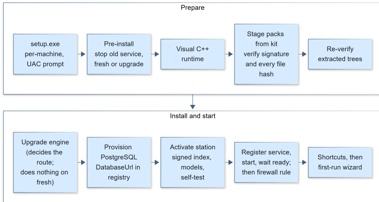
Figure 76: Installation and activation. A failure after the new files are in place tries to stop the service and set it to manual start (best effort), then exits with a numbered code.
