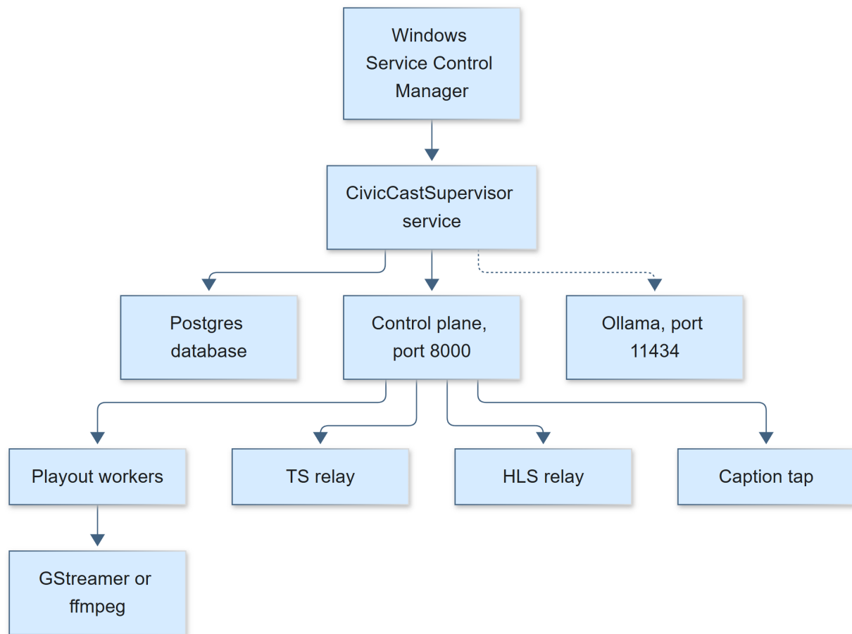
Figure 62: The processes CivicCast runs. A solid arrow means the parent starts and restarts the child; the dotted arrow means the child is optional.
