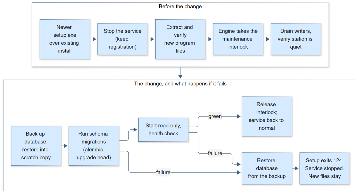
Figure 77: Upgrade and rollback.
