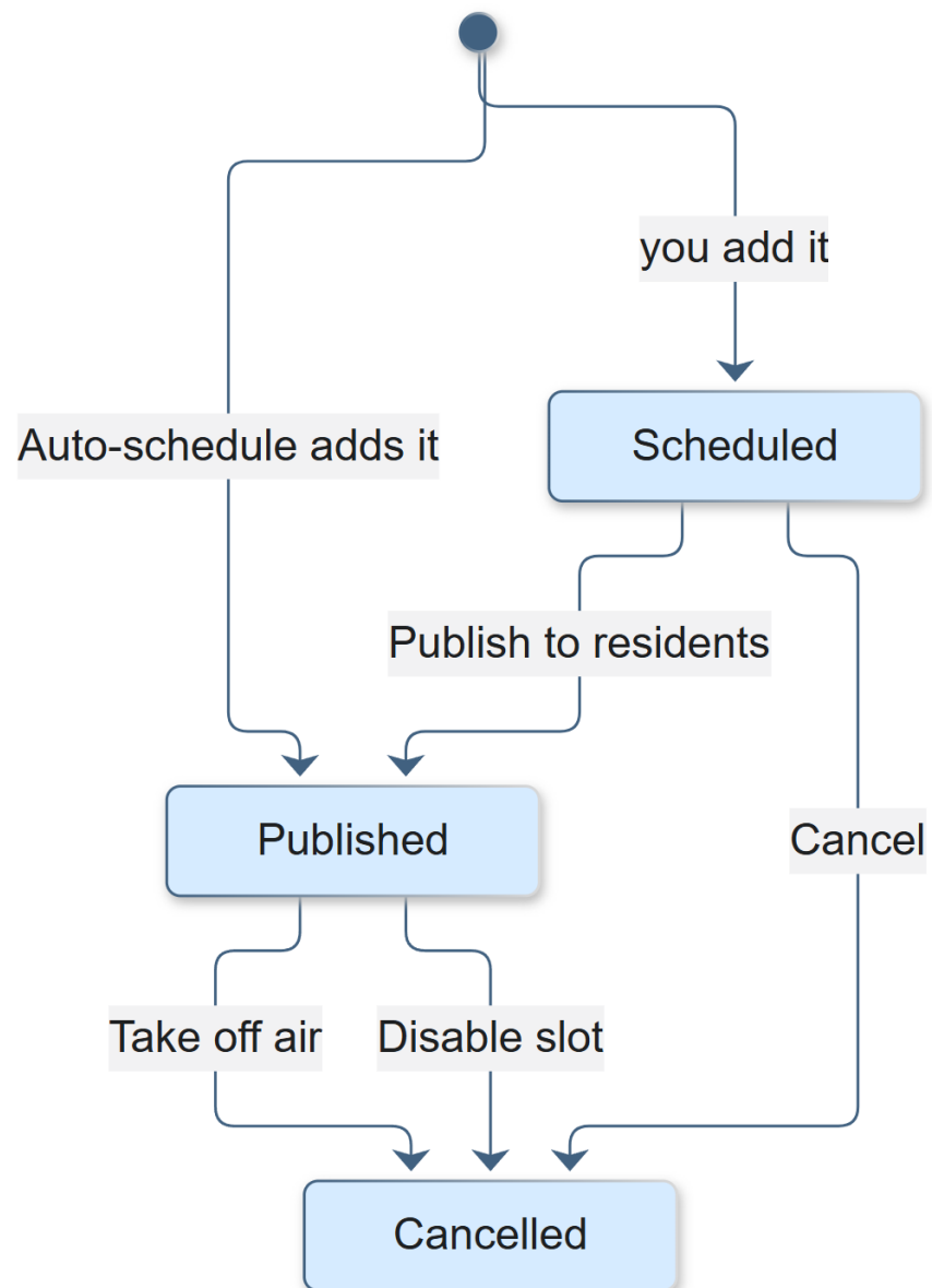
Figure 7: The life of a schedule item. Items you add by hand start as Scheduled. Items that Auto-schedule adds start as Published.
