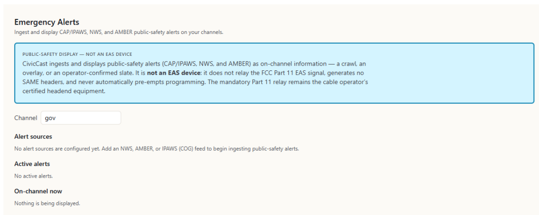
Figure 55: The Emergency Alerts screen. The permanent banner “Public-safety display — not an EAS device” sits above the Channel picker and the Alert sources, Active alerts and On-channel now lists.
