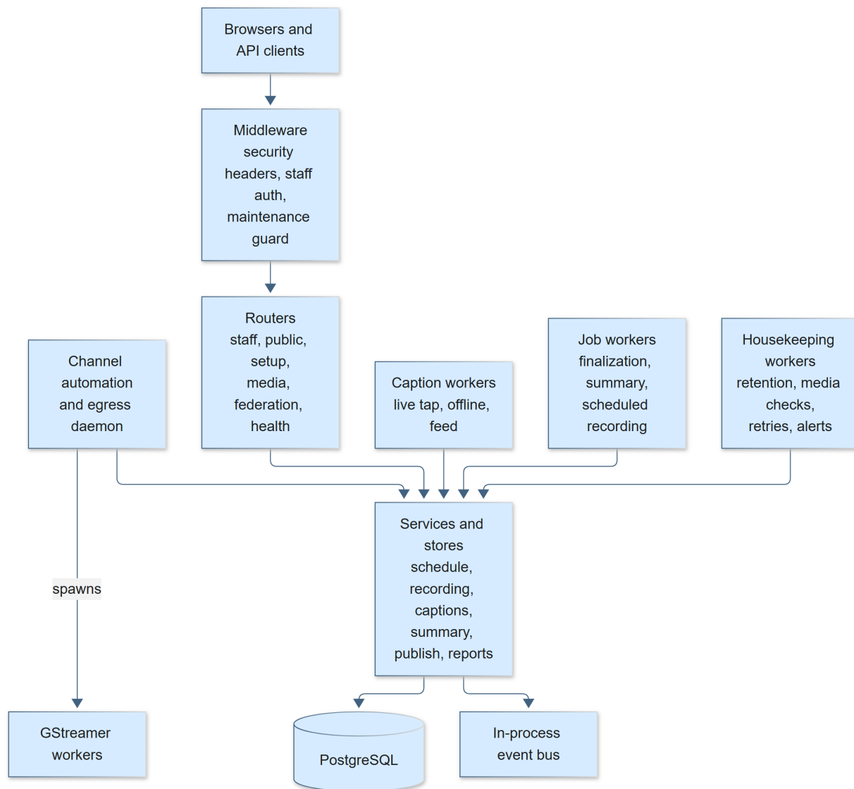
Figure 66: Parts of the control plane. The background workers are threads inside the same process as the web server; only the video workers are separate programs.
