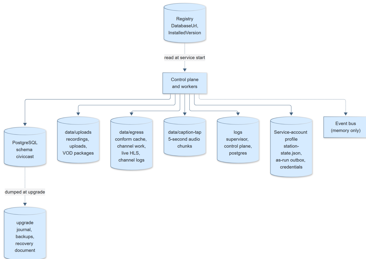
Figure 67: Data stores. The folders data, logs and upgrade are under C:\ProgramData\CivicCast. The registry values are under HKLM\SOFTWARE\CivicCast\Native.
