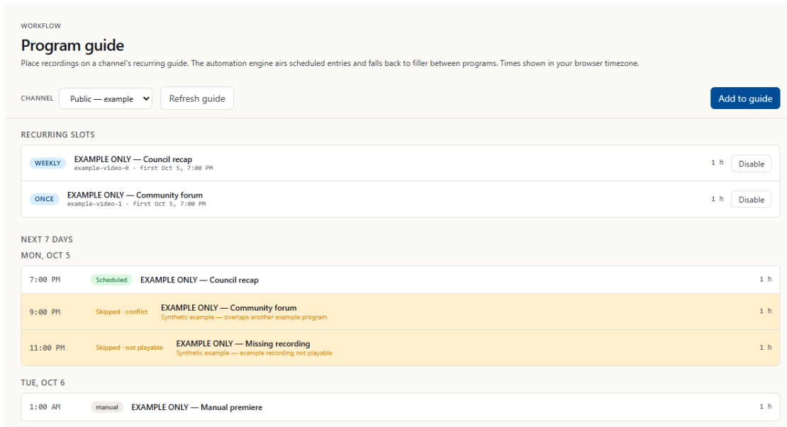
Figure 12: The Program guide screen with two recurring slots and the Next 7 days list.
