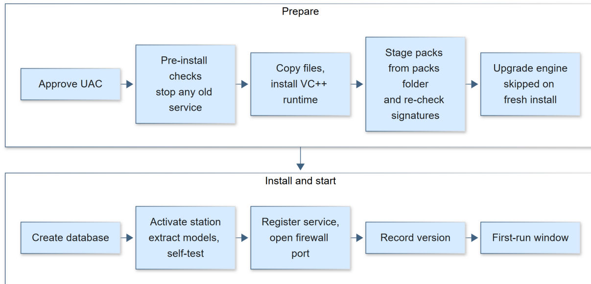
Figure 58: The order of the Windows setup steps and the first-run window.
