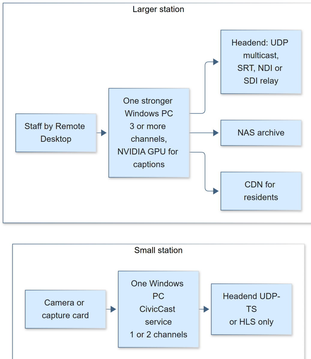
Figure 79: Two reference topologies. Both are one computer; the larger one adds equipment around it.
