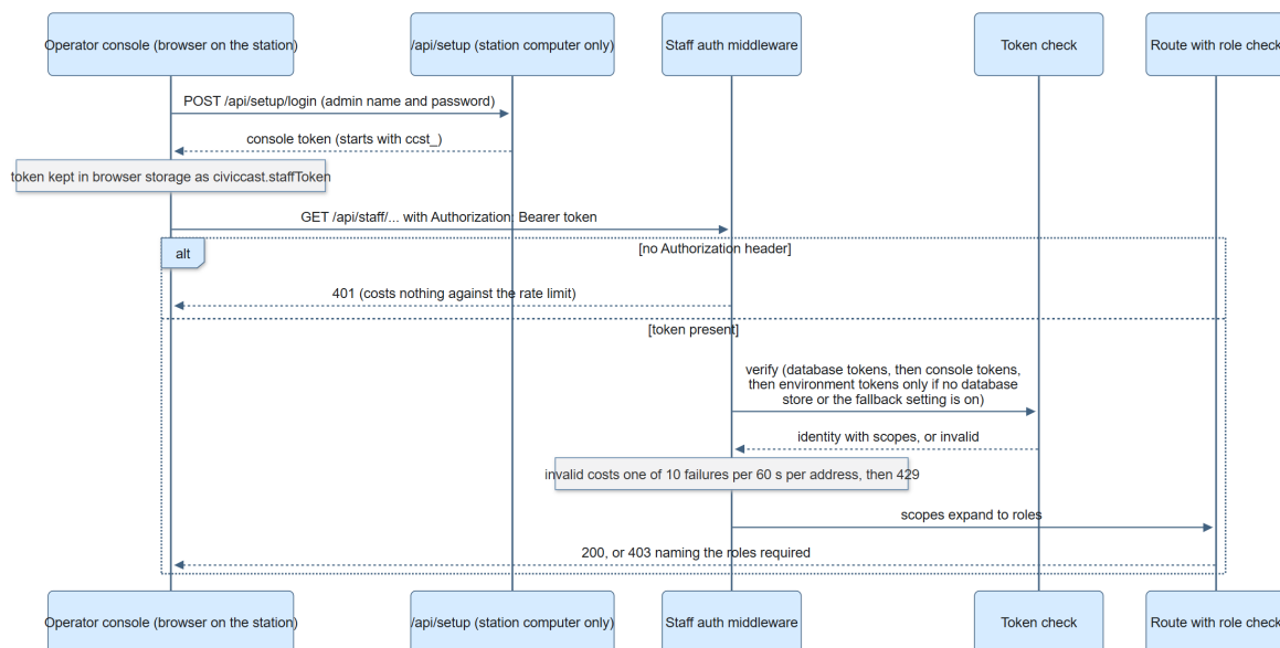
Figure 75: Sign-in and request authorization.
