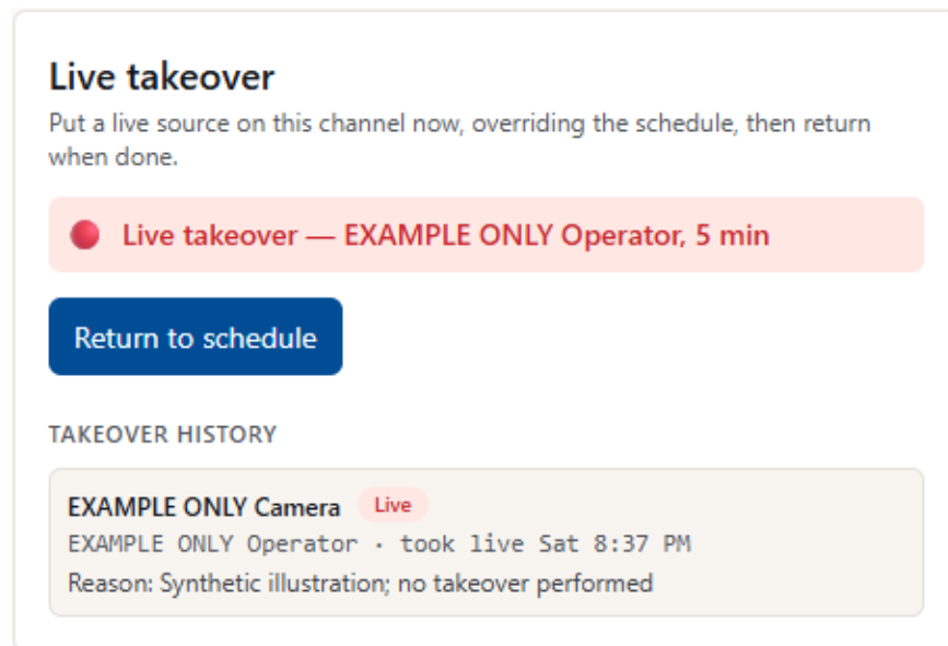
Figure 26: The Live takeover box while a channel is under takeover, with the Return to schedule button.
