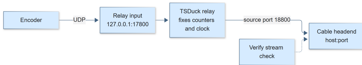
Figure 63: The path of a udp-ts output with the relay on. The encoder sends to a loopback address on the station; the relay forwards to the headend you configured.
