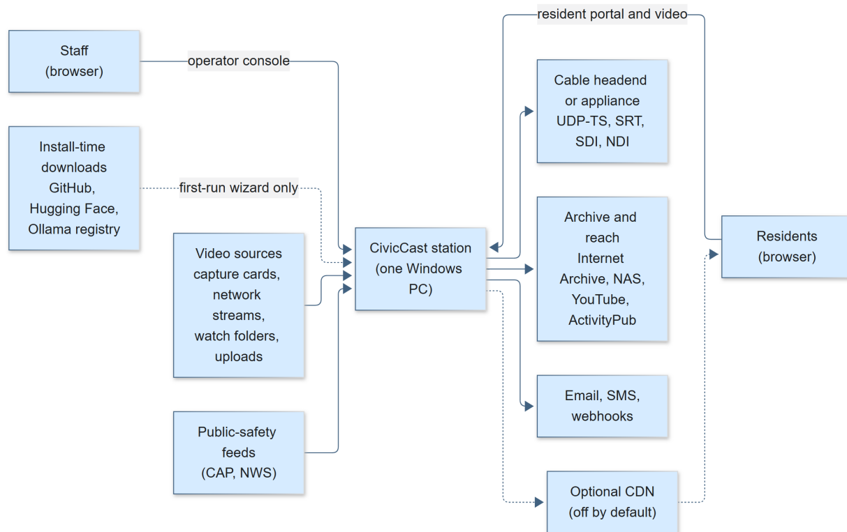
Figure 64: System context. Solid arrows are the normal flows. Dashed arrows are optional or occur only at install time.
