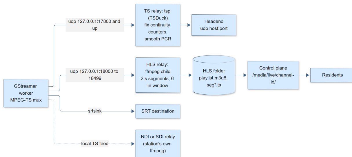
Figure 74: Output paths for one channel. The TS relay is used only for udp-ts sinks and only if TSDuck is present. A file sink writes the TS stream straight to a file, and is not shown.
