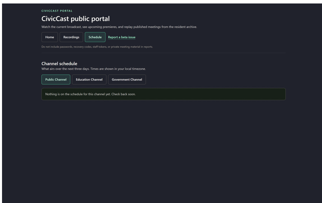
Figure 43: The Schedule page with channel buttons. The channel shown has no entries yet.
