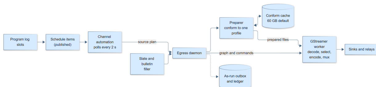
Figure 69: The playout pipeline for one channel. The daemon, the preparer and the automation run inside the control plane; the worker is a separate program.
