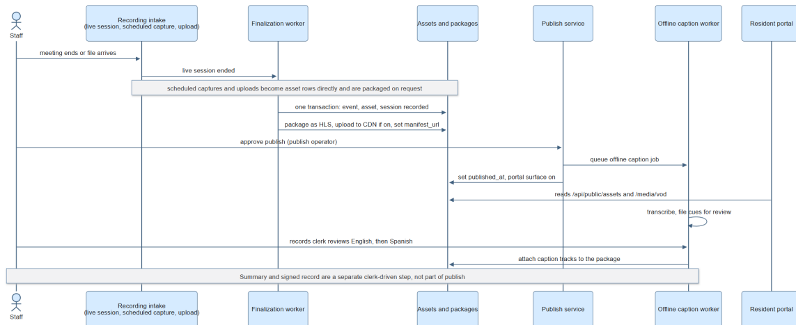
Figure 68: A recording from capture to resident. Captions are attached after the portal goes live.
