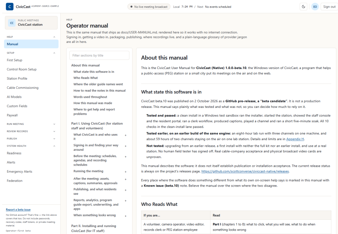
Figure 4: The operator console with a signed-in user. The top bar is across the top, and the sidebar on the left shows its six sections.
