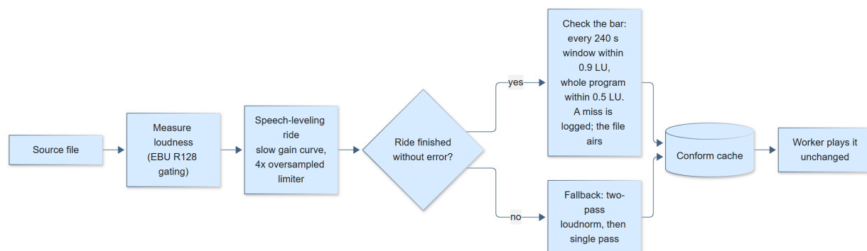
Figure 72: How program audio is leveled. The target is -16 LUFS by default.
