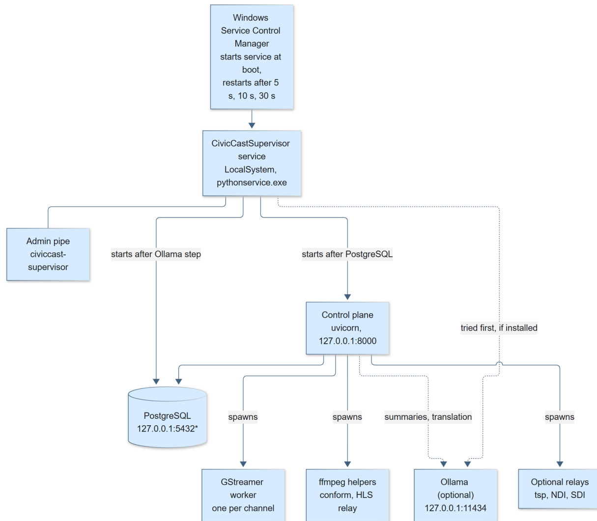
Figure 65: Processes on a native Windows station. *PostgreSQL uses the first free port of 5432, 5433, 5434, 5435 and 5544, chosen when the database was created.
