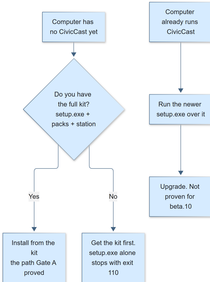
Figure 57: Which delivery you need. Only the full-kit path was proven in beta.10.
