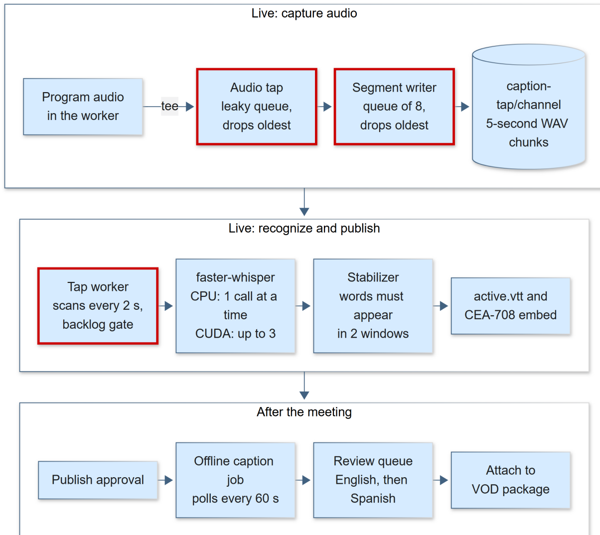
Figure 73: The caption pipelines. Boxes with a heavy red outline are where live audio can be shed under load. The offline path sheds nothing.
