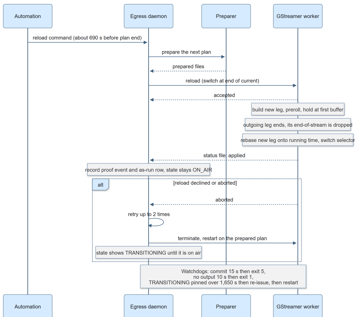
Figure 70: A program change (a “seamless reload”) and its watchdogs.
