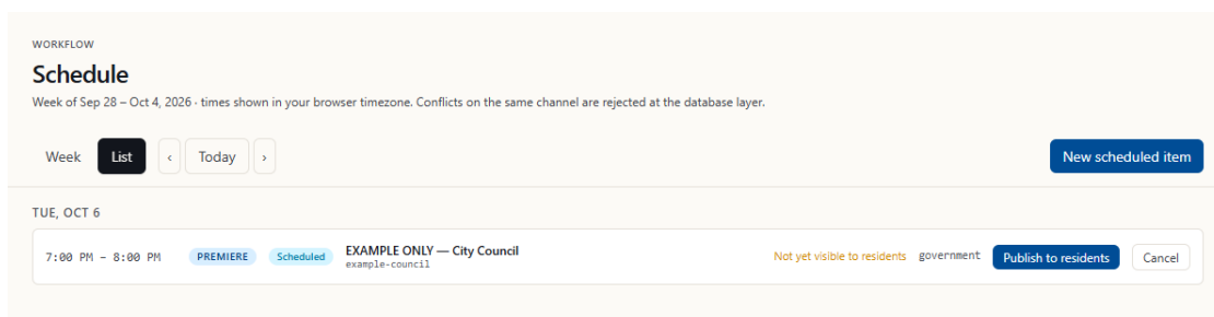
Figure 10: The Schedule list with one program waiting for approval. The row reads Not yet visible to residents and has a Publish to residents button.
