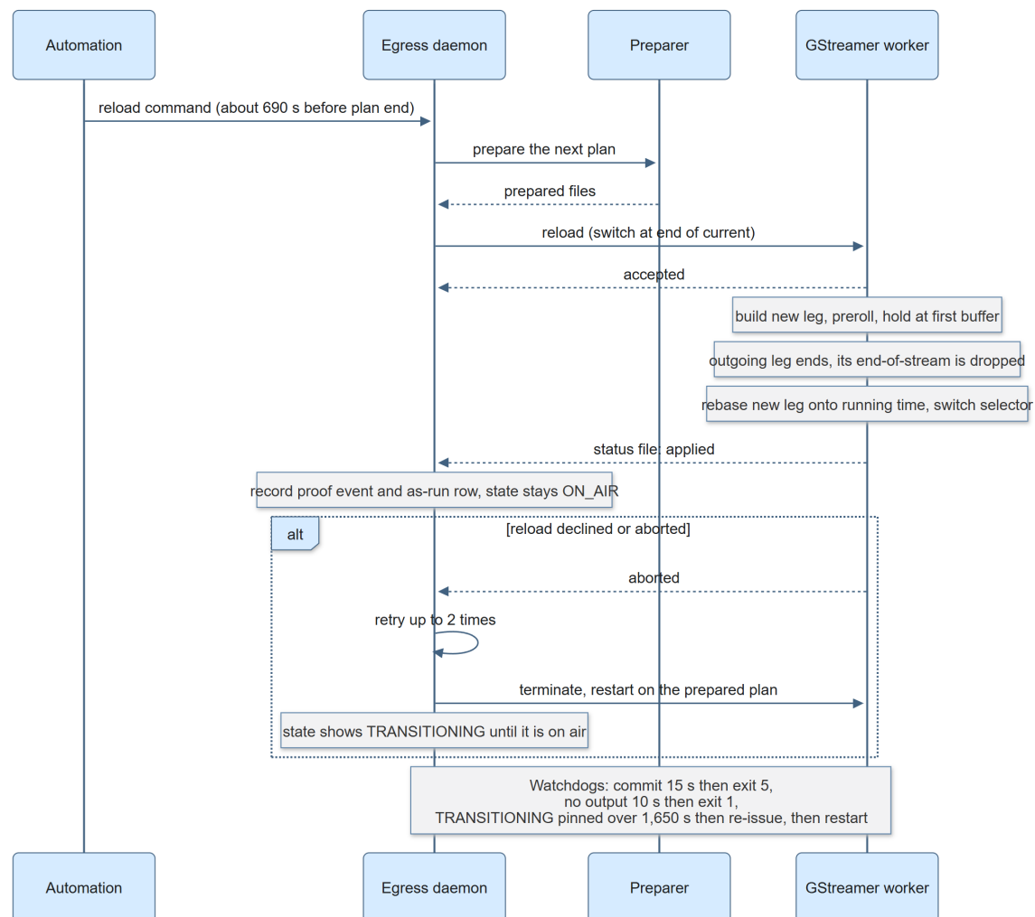
Figure 16-7. A program change (a “seamless reload”) and its watchdogs.
