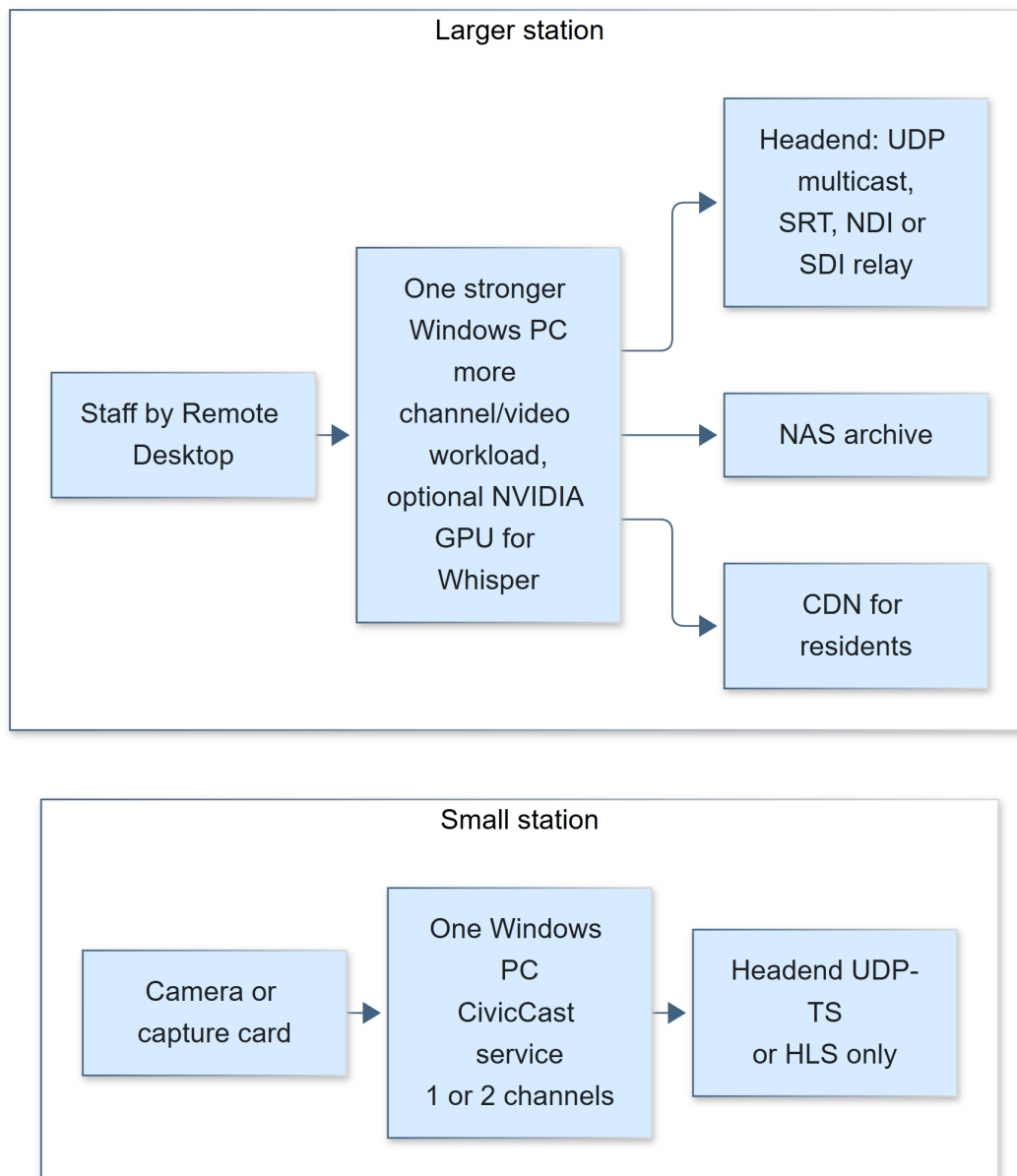
Figure 16-16. Two reference topologies. Both are one computer; the larger one adds equipment around it.
