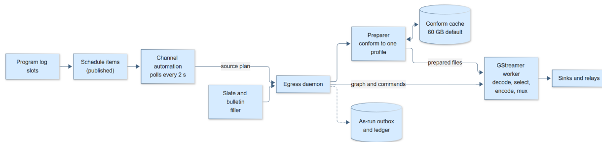
Figure 16-6. The payout pipeline for one channel. The daemon, the preparer and the automation run inside the control plane; the worker is a separate program.
