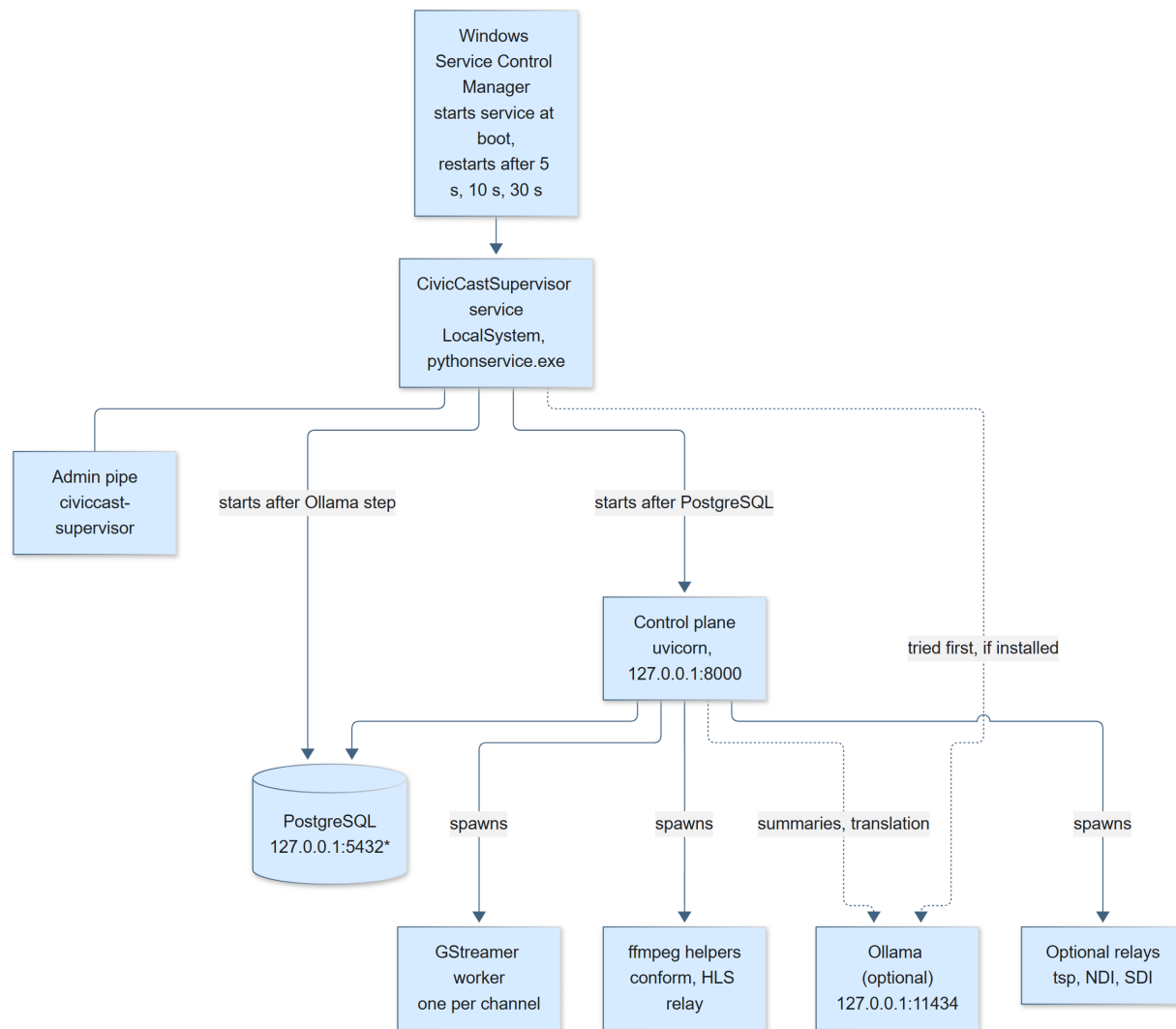
Figure 16-2. Processes on a native Windows station. *PostgreSQL uses the first free port of 5432, 5433, 5434, 5435 and 5544, chosen when the database was created.
