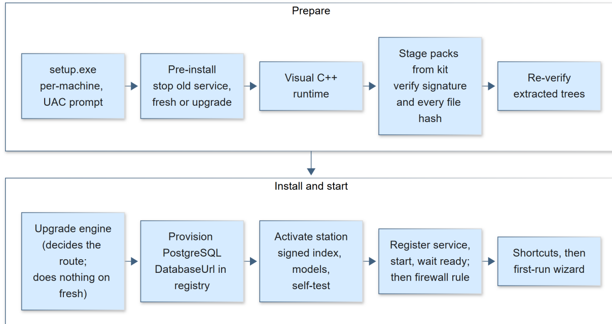
Figure 16-13. Installation and activation. A failure after the new files are in place tries to stop the service and set it to manual start (best effort), then exits with a numbered code.
