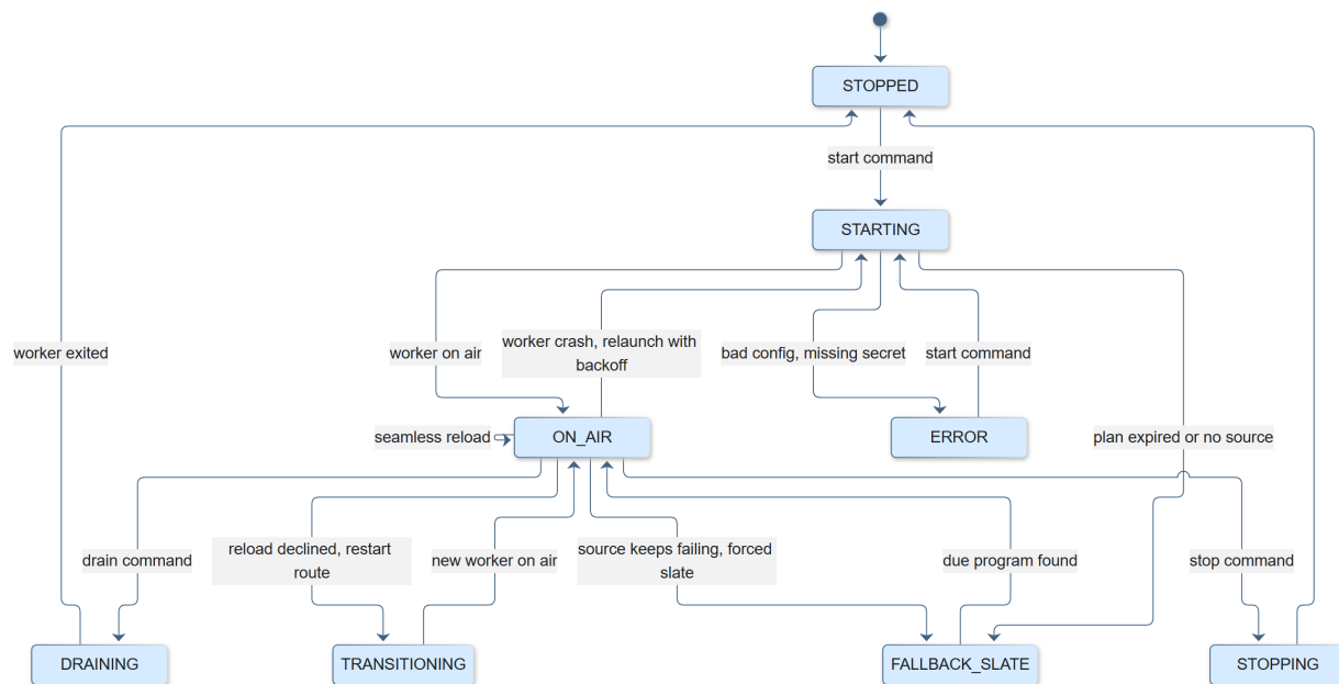
Figure 16-8. Channel states. The state is written by the egress daemon.
