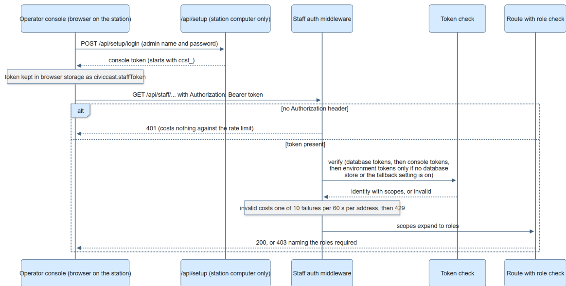
Figure 16-12. Sign-in and request authorization.
