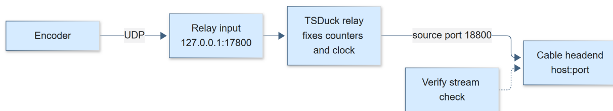
Figure: the path of a udp-ts output with the relay on. The encoder sends to a loopback address on the station; the relay forwards to the headend you configured.
