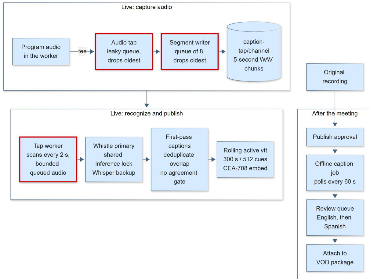
Figure 16-10. The caption pipelines. Boxes with a heavy red outline are where live audio can be shed under load. The offline path sheds nothing.
