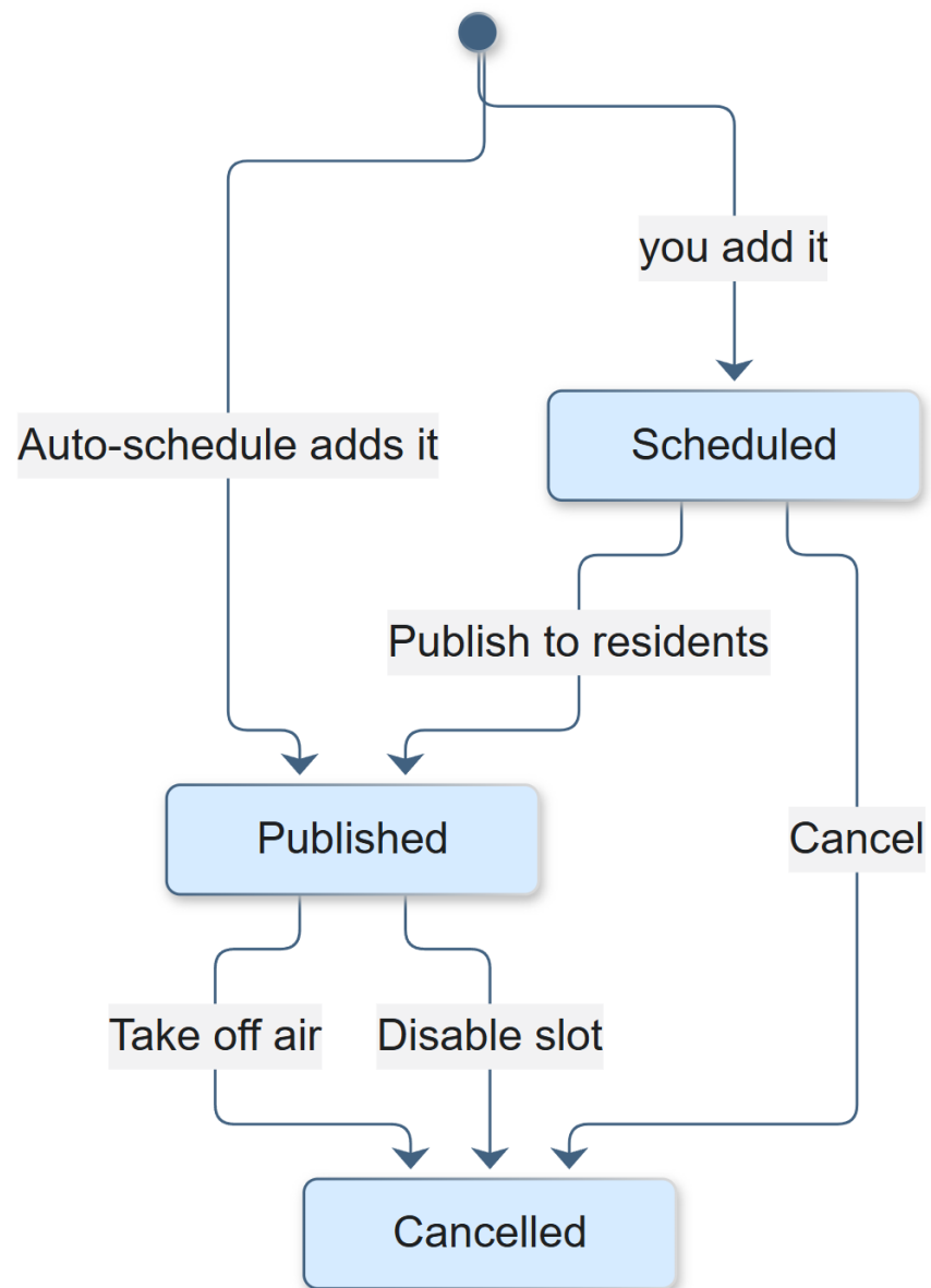
Figure: the life of a schedule item. Items you add by hand start as Scheduled. Items that Auto-schedule adds start as Published.
