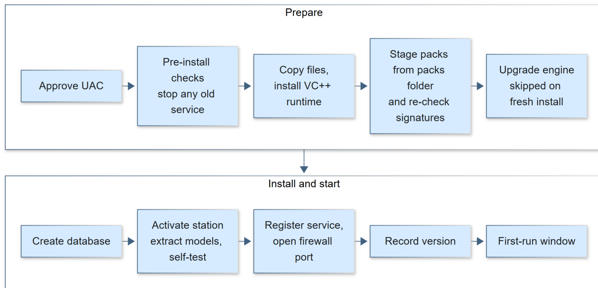
Figure 10.1. The order of the Windows setup steps and the first-run window.
