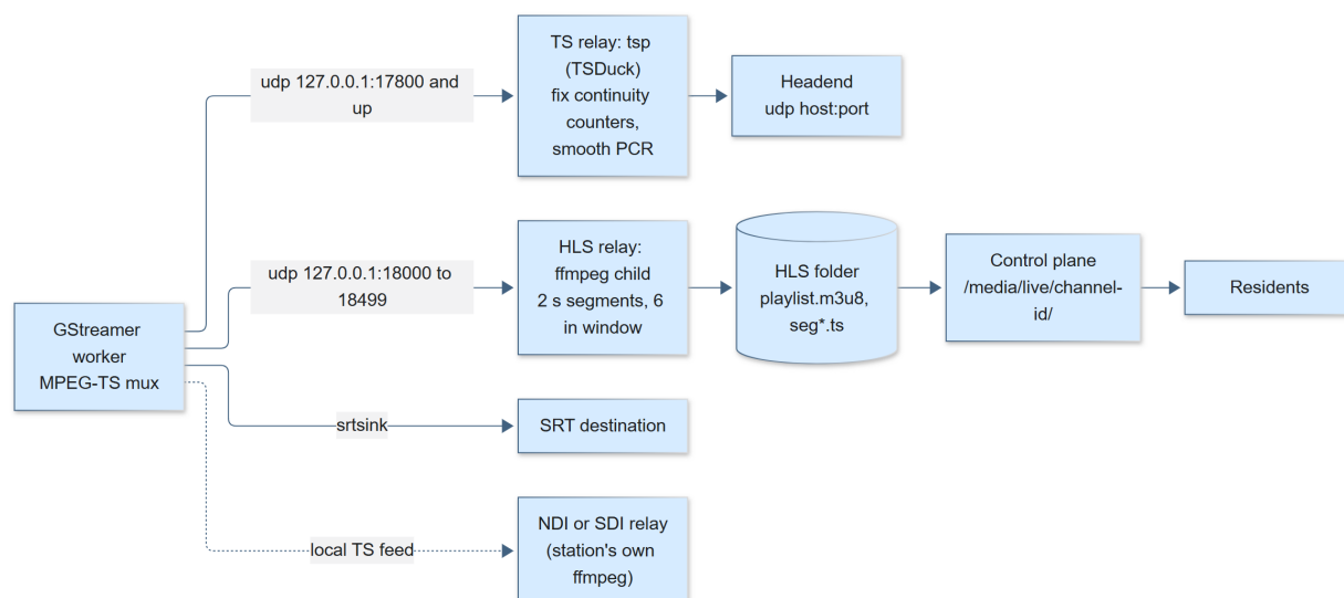
Figure 16-11. Output paths for one channel. The TS relay is used only for udp-ts sinks and only if TSDuck is present. A file sink writes the TS stream straight to a file, and is not shown.
