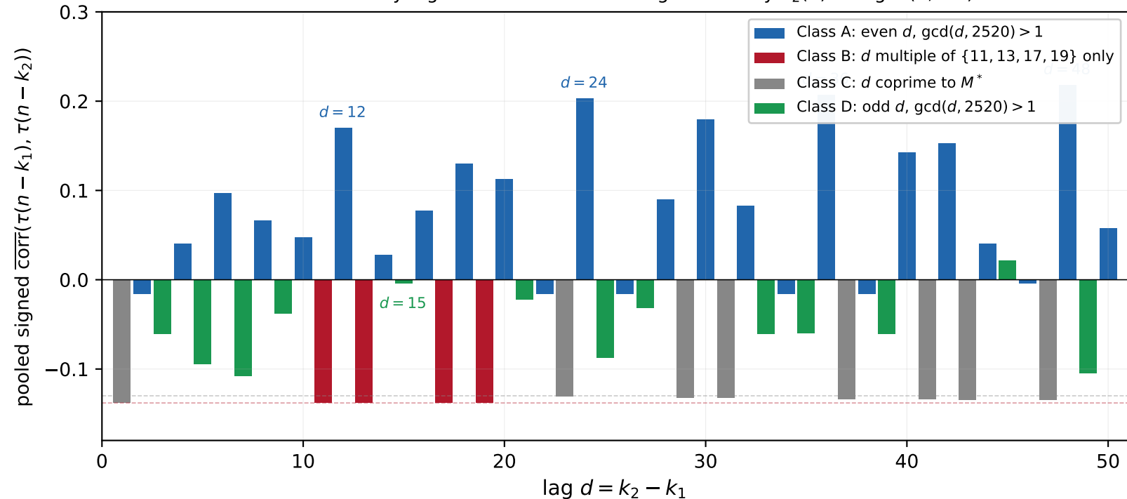
\tau -correlation by lag — four-class structure governed by v_2(d) and \gcd(d, M^*)
