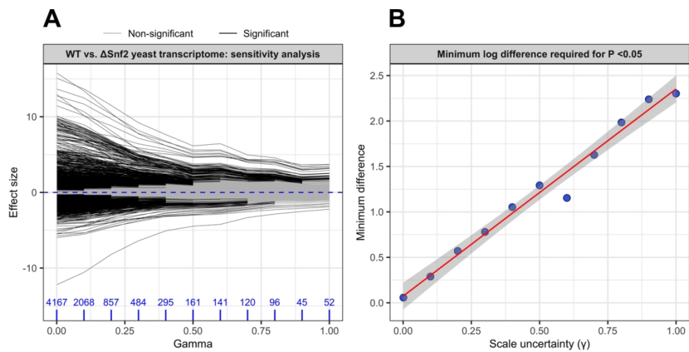
Sensitivity analysis informs the selection of an appropriate gamma value: Count data from the yeast transcriptome dataset was used for a sensitivity analysis in ALDEx2, using a range of gamma values from 0 to 1.0 in increments of 0.1. (A) Effect sizes at each gamma value are plotted for all features and coloured by significance at each gamma value. Blue numbers indicate the number of differentially expressed features at each gamma value. (B) The minimum absolute log difference between wild-type and Snf2 knockout cells required for a statistically significant result is shown for each gamma value. Regression line represents a slope of 2.2.
