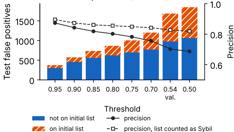
A Test false positives (baseline)
