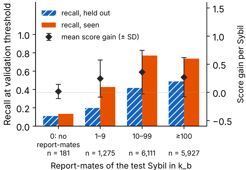
A Dose-response (LightGBM)
