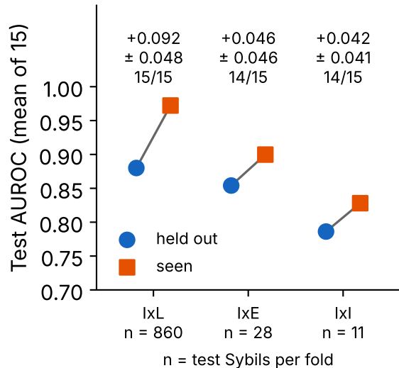
B AUROC by category (LightGBM)
