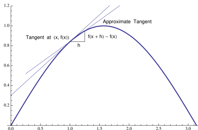
Figure 3.7: Tangent and approximating tangent.
