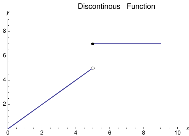
Figure 3.8: This function does not have a tangent line at (5, f(5)) .
