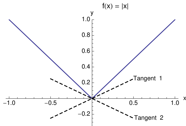
Figure 3.10: No unique tangent line at (0, f(0)) = (0, 0) . Two possible tangents are drawn with dashed lines.
