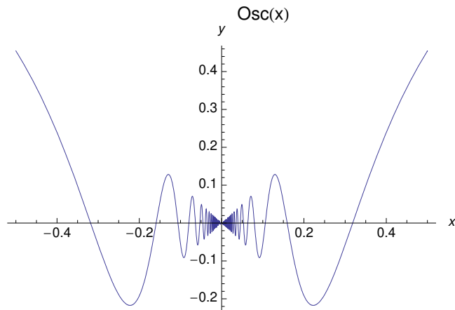
Figure 3.9: The function \text{Osc}(x) = \begin{cases} x \sin(1/x) & \text{if } x \neq 0 \\ 0 & \text{if } x = 0 \end{cases} has no tangent at (0, \text{Osc}(0)) .
