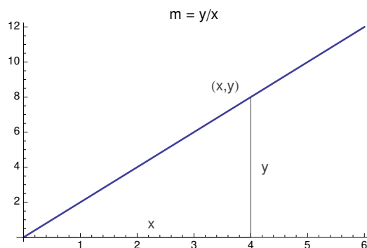
Figure 2: A linear function.
