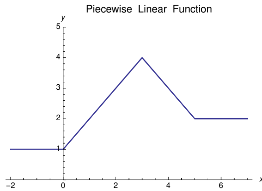
Figure 2: A sample piecewise linear function.
