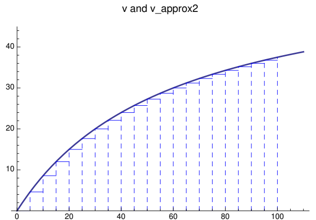
Figure 4.4: A better approximation to v .
