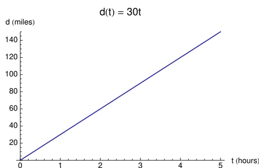
Figure 3.12: Distance graph when car is traveling 30 mph.
