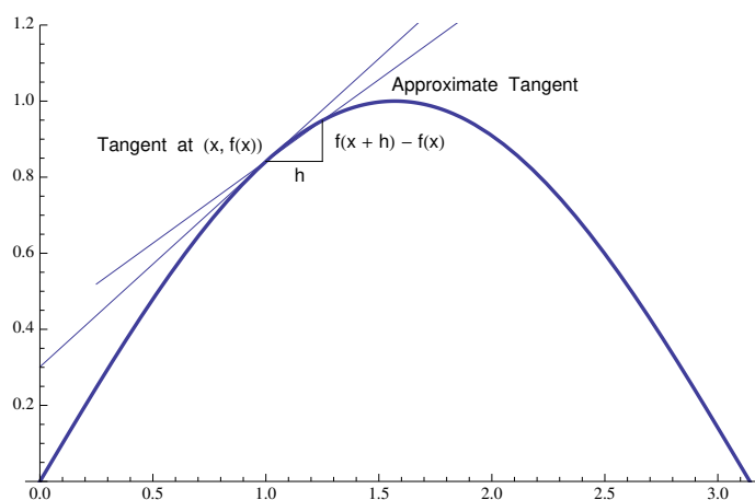
Figure 3.7: Tangent and approximating tangent.
