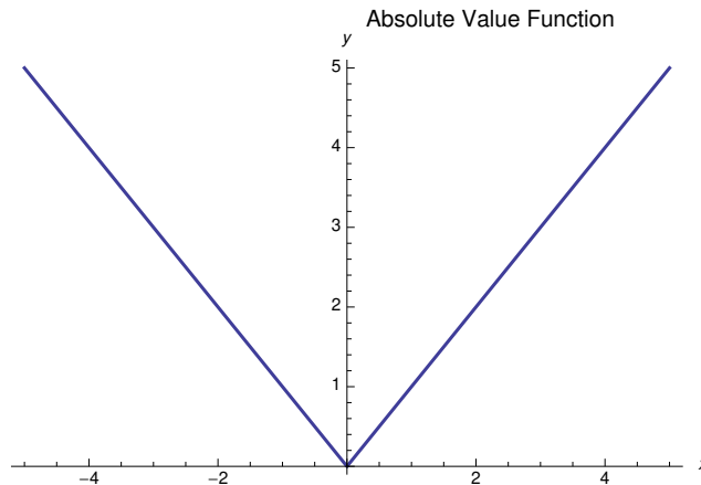
Figure 1: The absolute value function f(x) = |x| .
