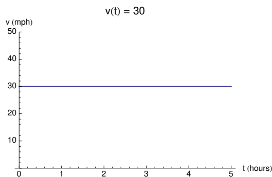
Figure 3.13: Velocity graph when car is traveling 30 mph.
