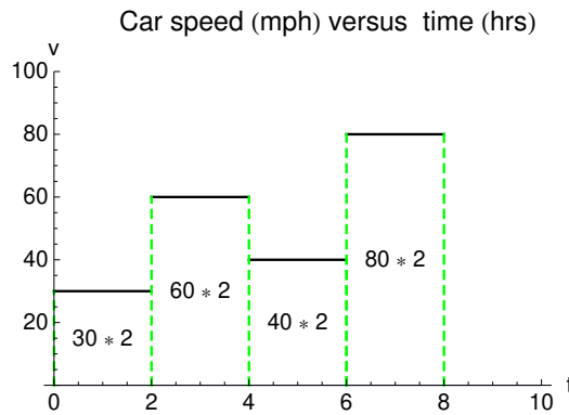
Figure 4.1: Piecewise constant velocity.
