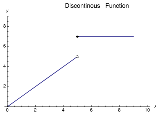
Figure 3: A discontinuous function.
