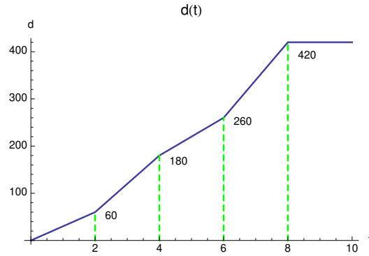
Figure 4.2: Piecewise linear distance function.
