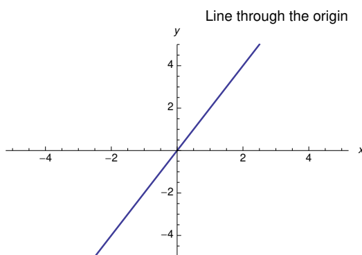
Figure 1: Straight line through the origin.
