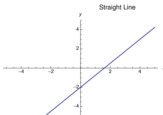
Figure 3: A straight line.
