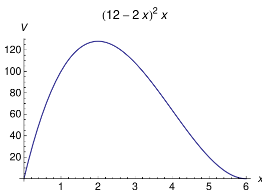
Figure 3.2: Box volume as a function of flap distance.
