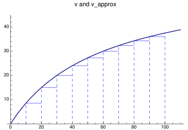
Figure 4.3: Piecewise constant approximation to velocity function, v .
