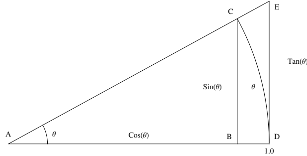
Figure 3.11: Comparison of triangle ABC, sector ADC, and triangle ADE.
