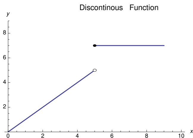
Figure 3.8: This function does not have a tangent line at (5, f(5)) . All of possible approximating slopes tend to \infty – not a number.
