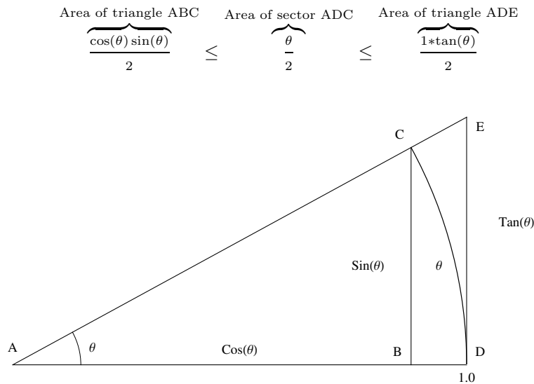
Figure 3.11: Comparison of triangle ABC, sector ADC, and triangle ADE.
