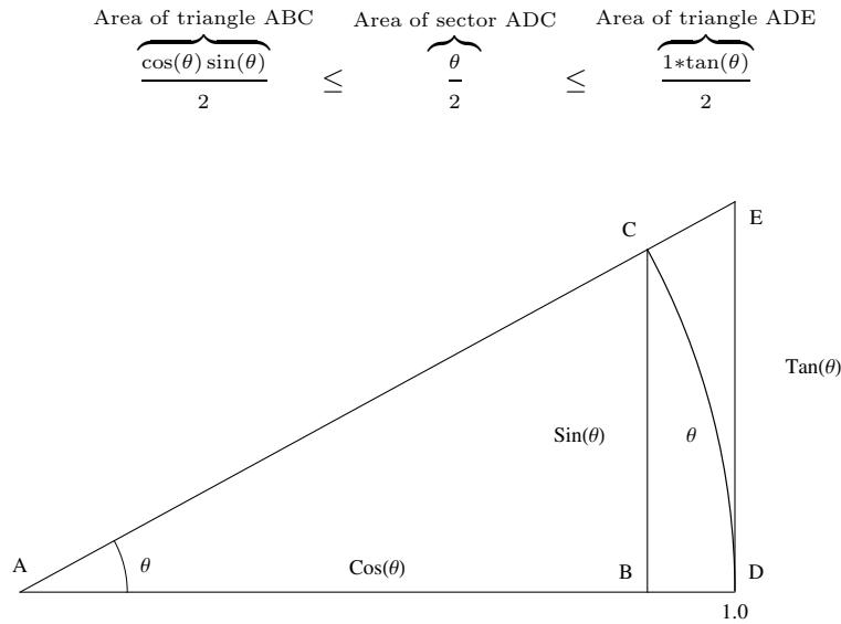
Figure 3.11: Comparison of triangle ABC, sector ADC, and triangle ADE.
