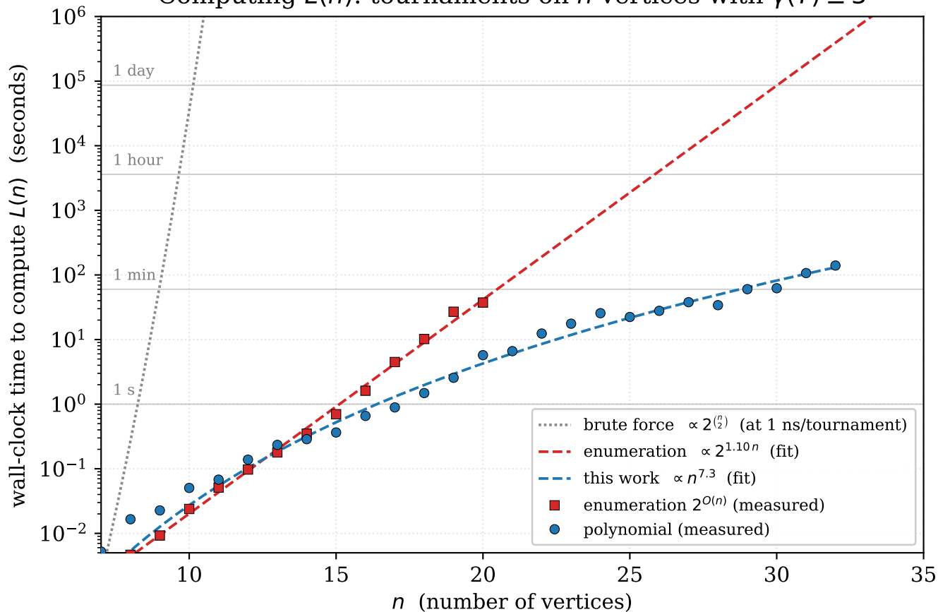
Computing L(n) : tournaments on n vertices with \gamma(T) \geq 3
