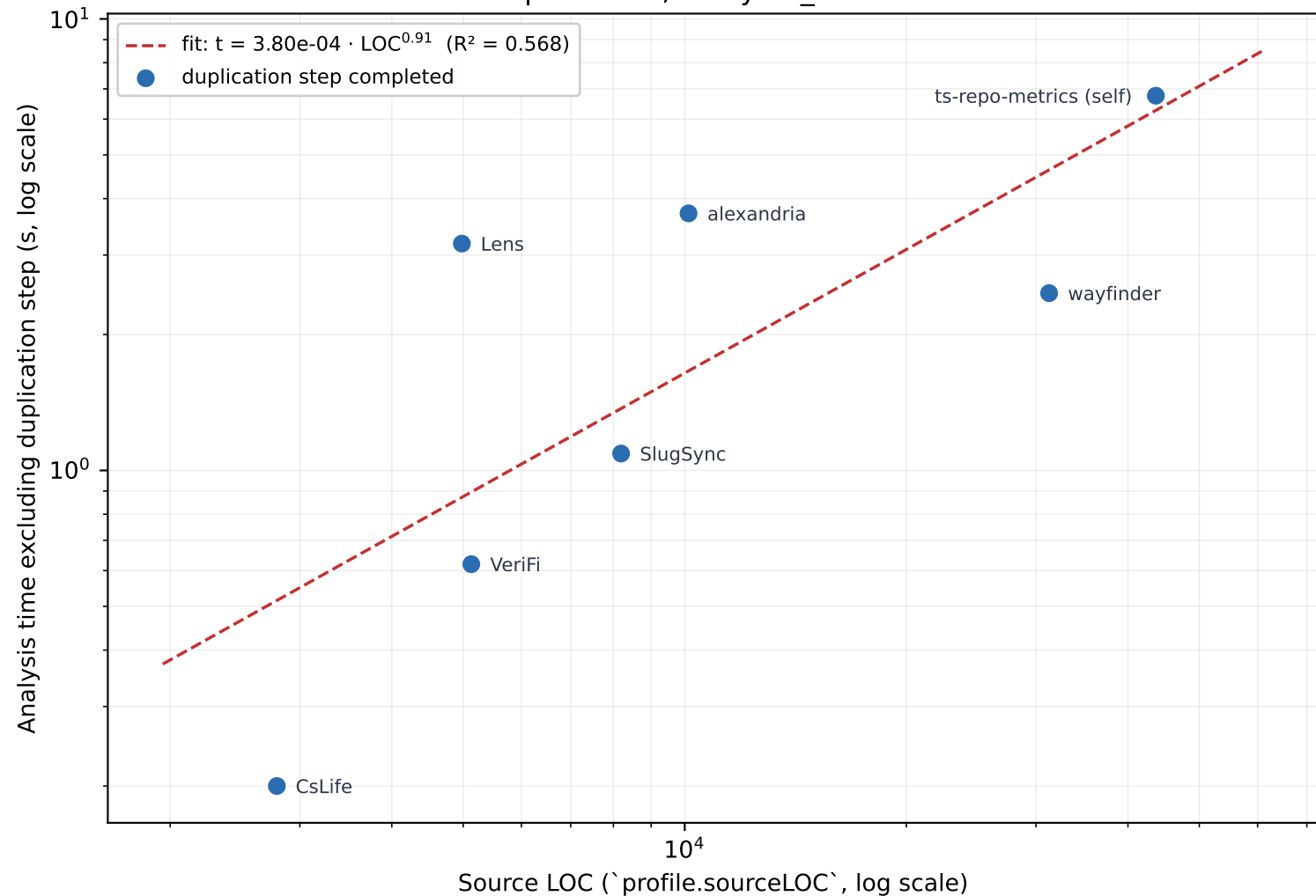
Figure 3 — Analysis time vs repository size n=7 repositories, analyzer_version 0.2.0
