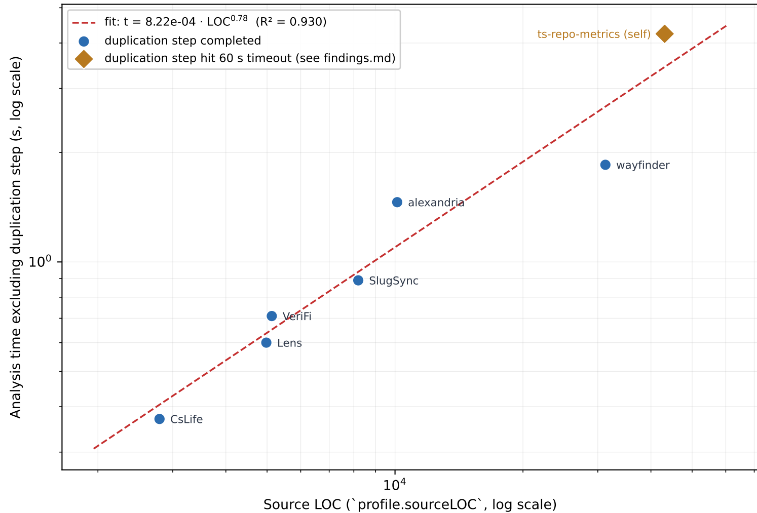
Figure 3 — Analysis time vs repository size n=7 repositories, analyzer_version 0.1.0
