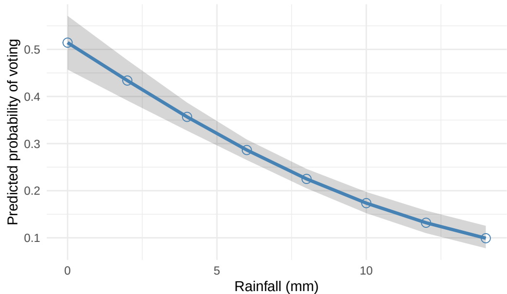
Predicted probability of voting by rainfall
