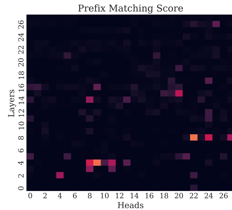
(f) Qwen2.5-VL-7B-Instruct (all tokens) 0.705
