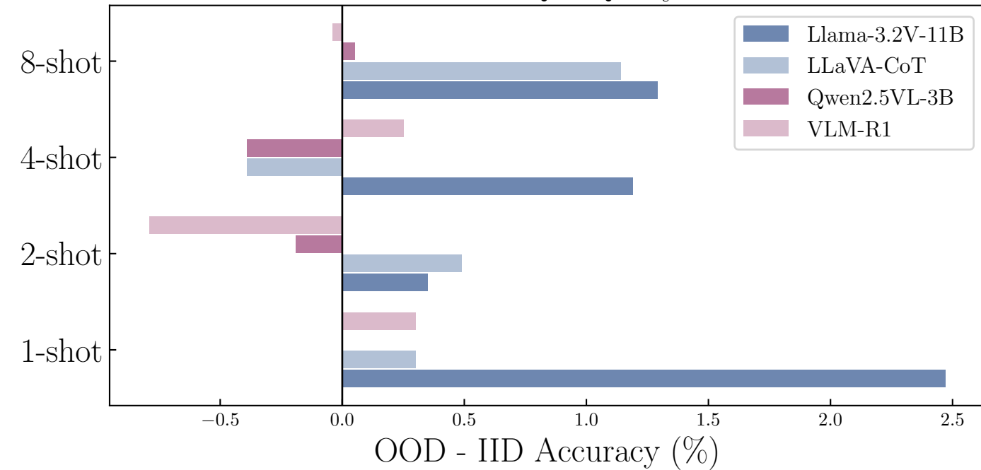
ScienceQA Query
