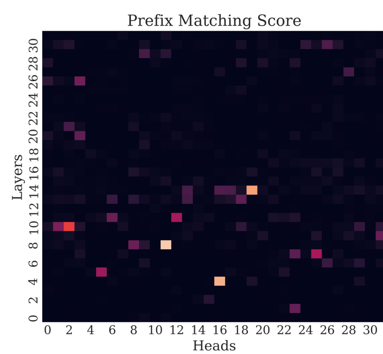
(b) Llama-3.2-11B-Vision-Instruct (all tokens) 0.916
