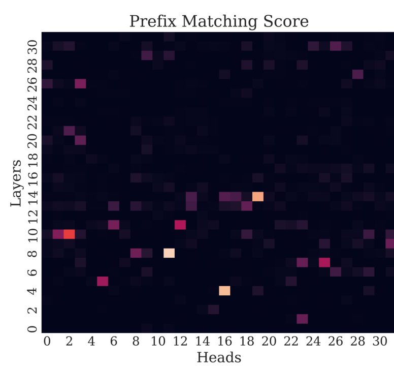
(c) Llama-3.2-11B-Vision-Instruct (text tokens) 0.937
