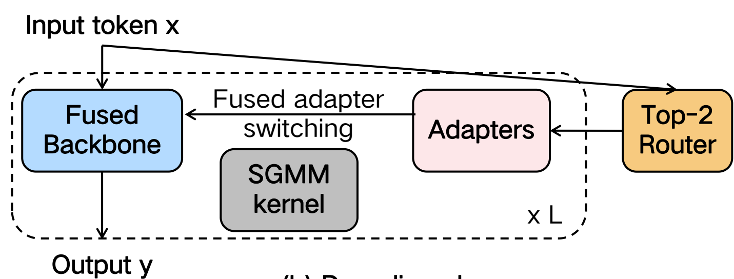
(b) Decoding phase
