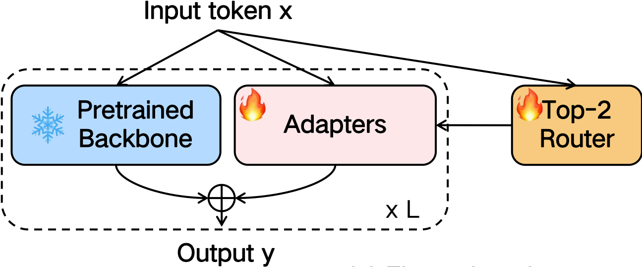
(a) Finetuning phase
