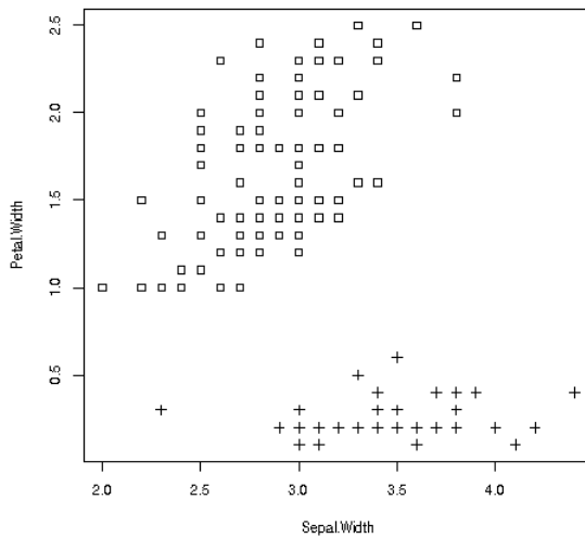
Figure 10-3: Setosa and nonsetosa
