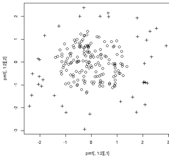
Figure 10-7: “Doughnut” data
