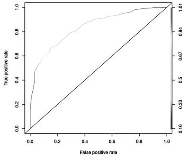
Figure 2-1: ROC, Telco Churn data
