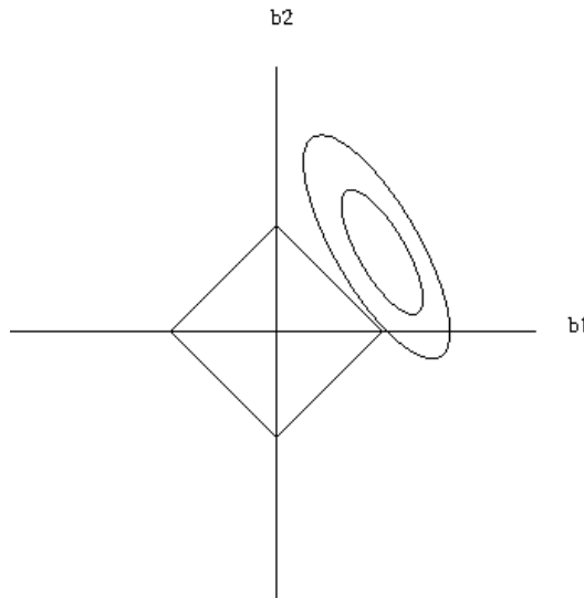
Figure 9-3: Feature subsetting nature of the LASSO
