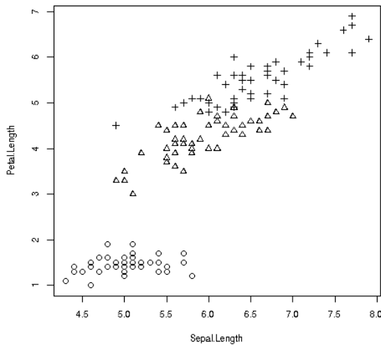
Figure 10-6: Iris data; three classes
