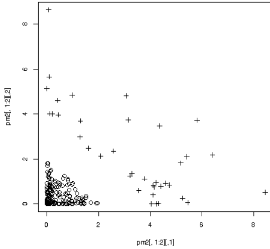
Figure 10-8: “Doughnut” data, transformed
