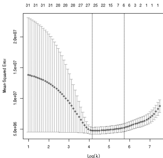
Figure 9-1: MSPE, Airbnb data
