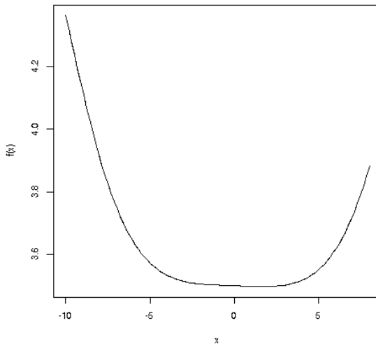
Figure 11-2: Shallow minimum region
