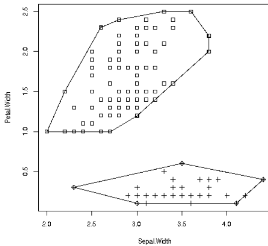
Figure 10-4: SVM convex hulls
