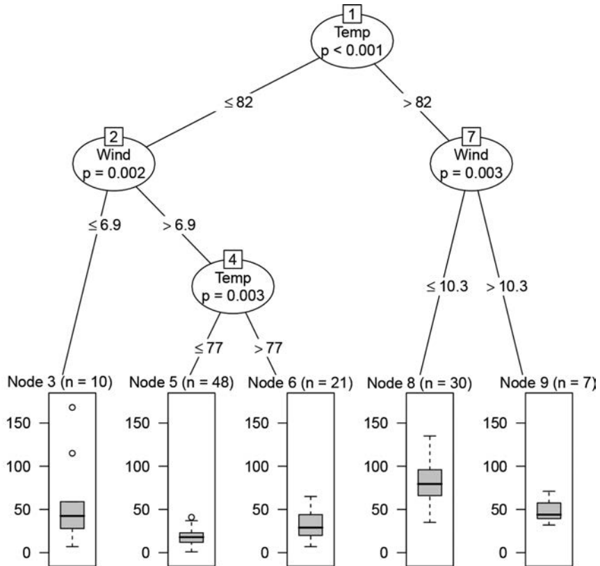
Figure 5-1: Sample plot from ctree
