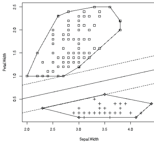
Figure 10-5: SVM margin
