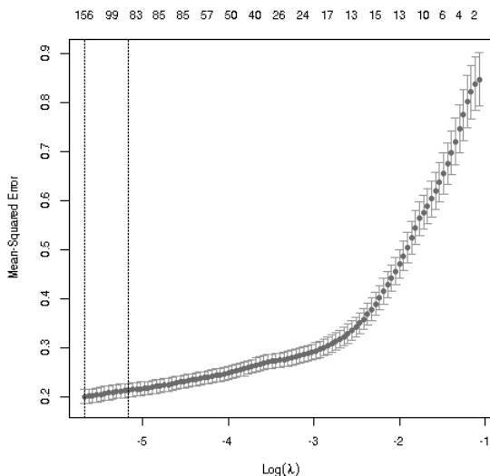
Figure 9-2: African soil data
