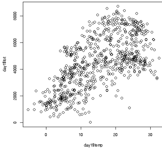
Figure 8-3: Ridership vs. temperature
