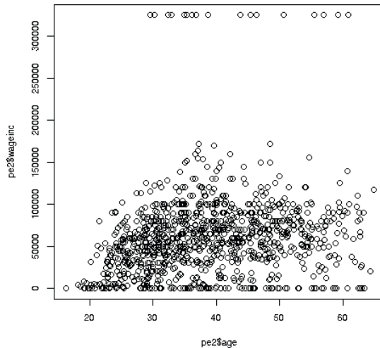
Figure 8-2: Wage income vs. age
