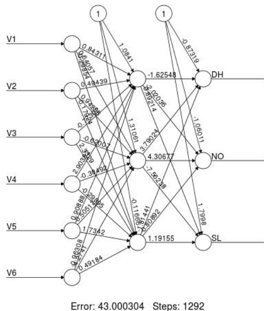
Figure 11-1: Vertebrae NN with one hidden layer
