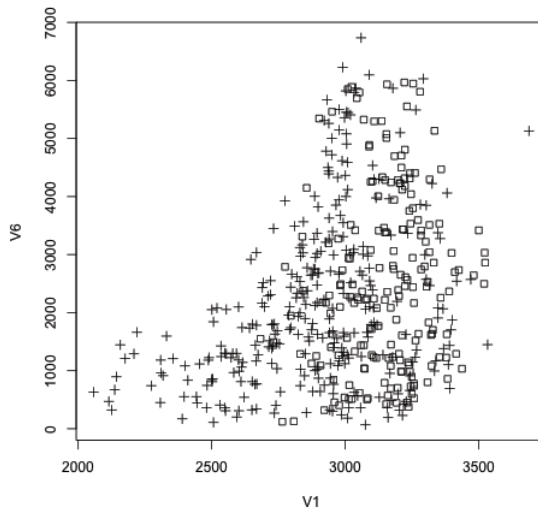
Figure 10-1: Forest cover data
