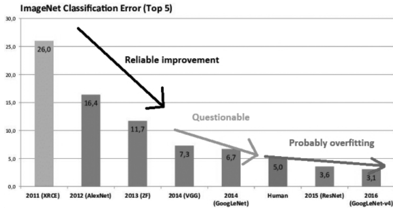
Figure D-1: AI p -hacking
