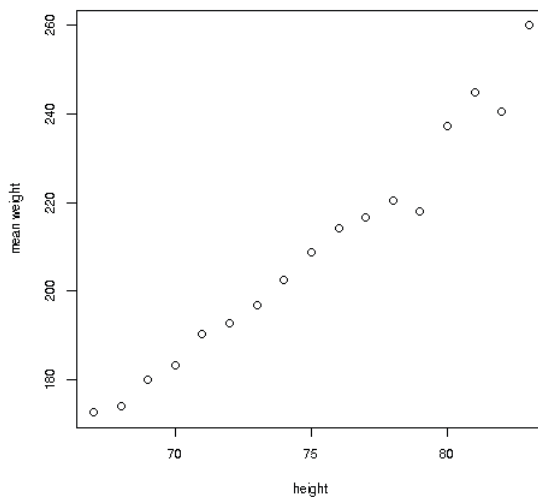
Figure 8-1: Estimated regression function, weight vs. height
