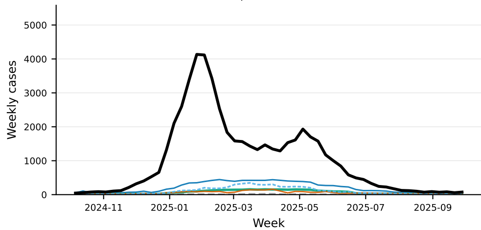
MT | WIS=704.8
