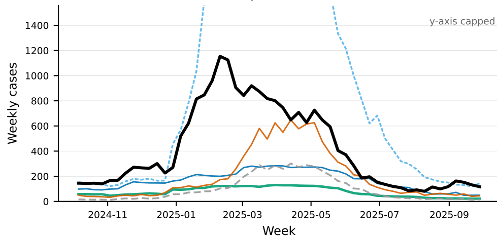
MG | WIS=154.3
