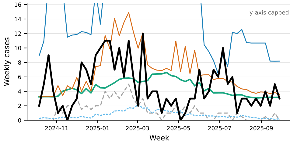
MG | WIS=154.3
