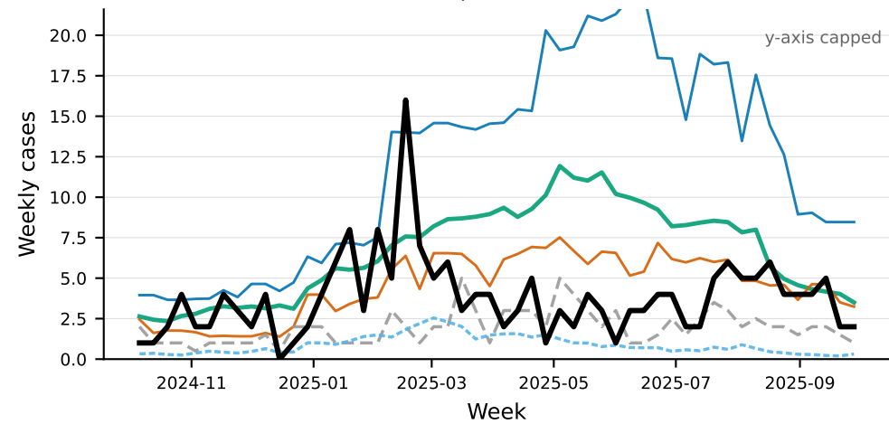
MT | WIS=704.8
