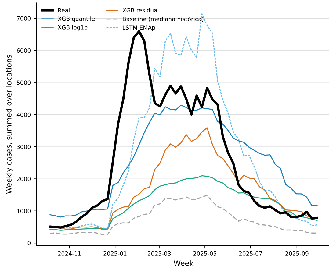
chikungunya_uf: validation_3 aggregate curve
