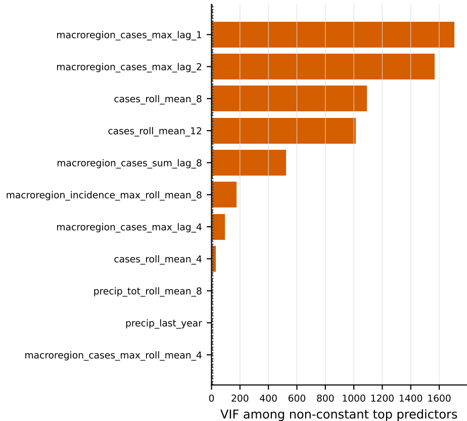
Collinearity diagnostic
