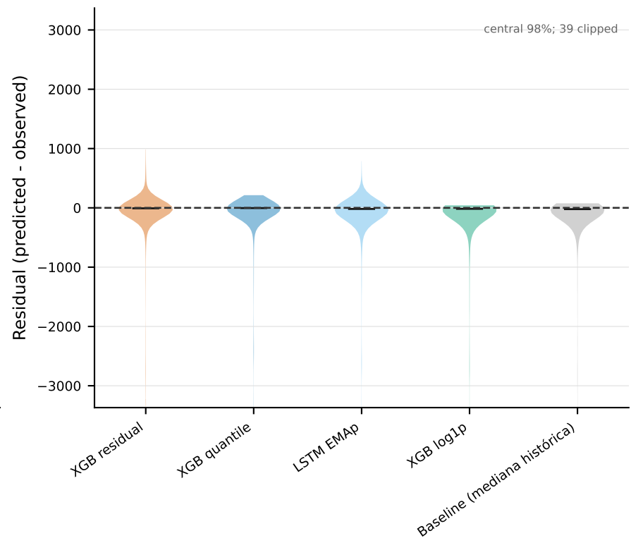
Residual distribution
