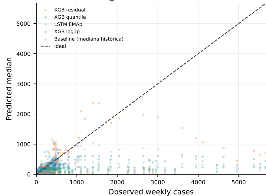
dengue_city: predicted vs observed
