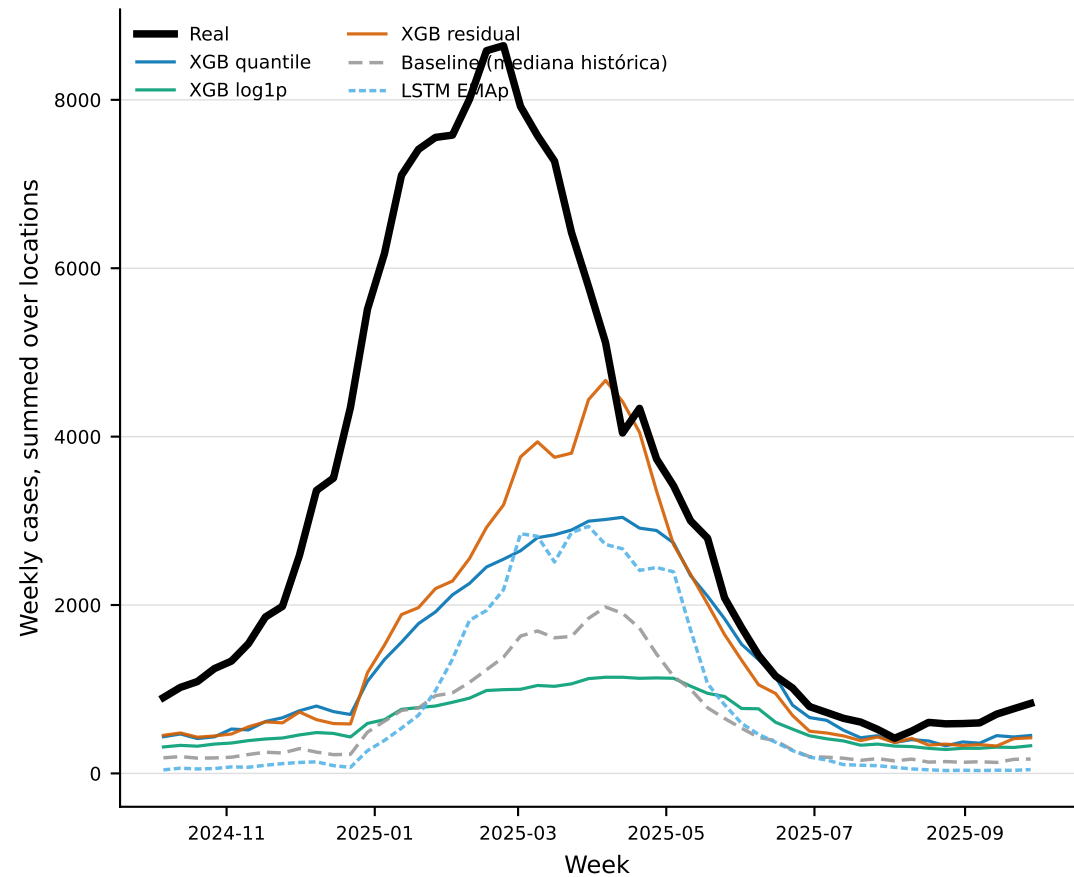
dengue_city: validation_3 aggregate curve
