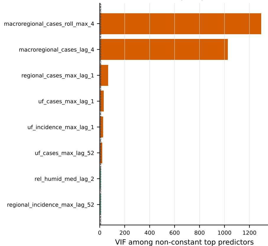
Collinearity diagnostic
