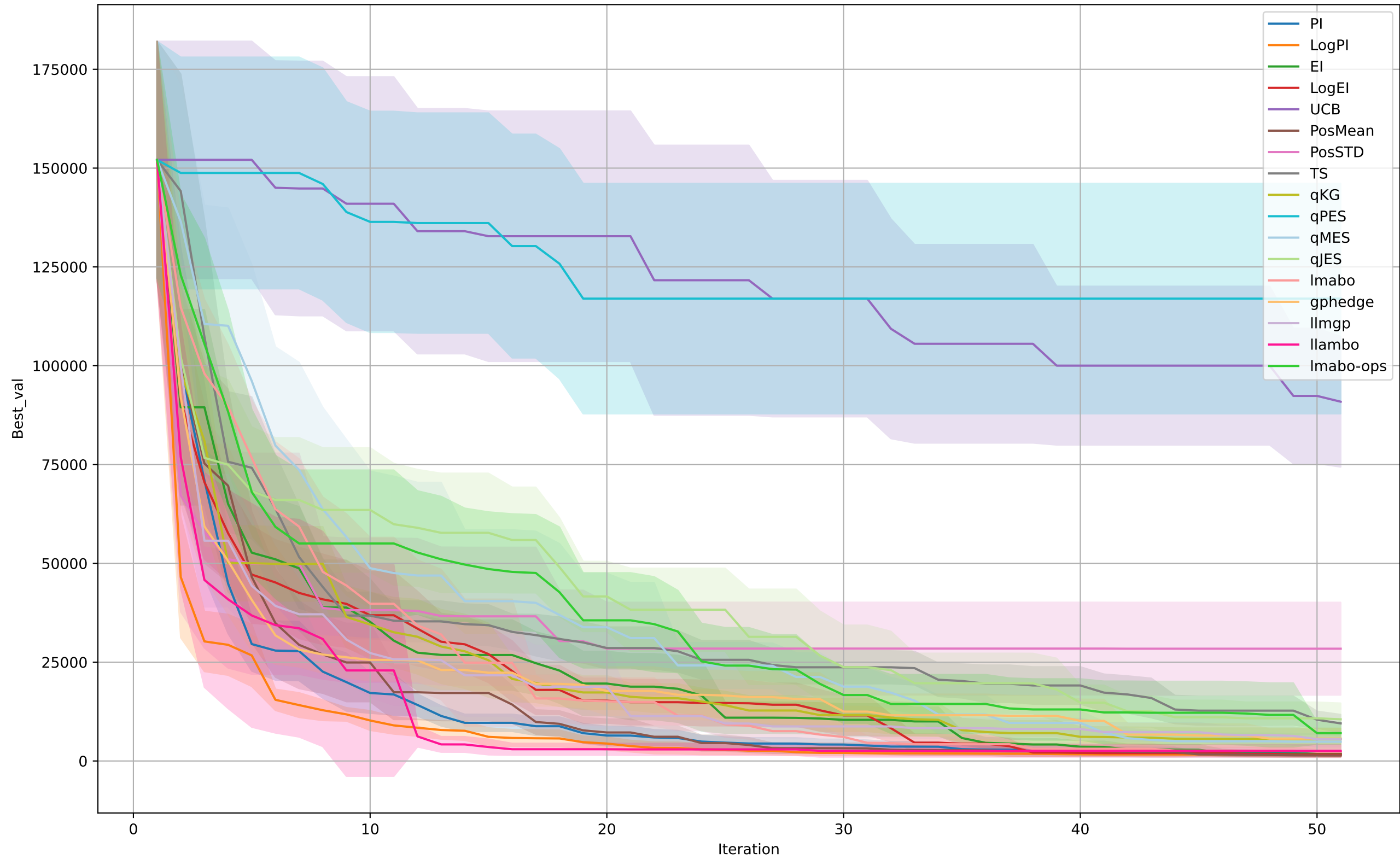
RosenbrockRotated
