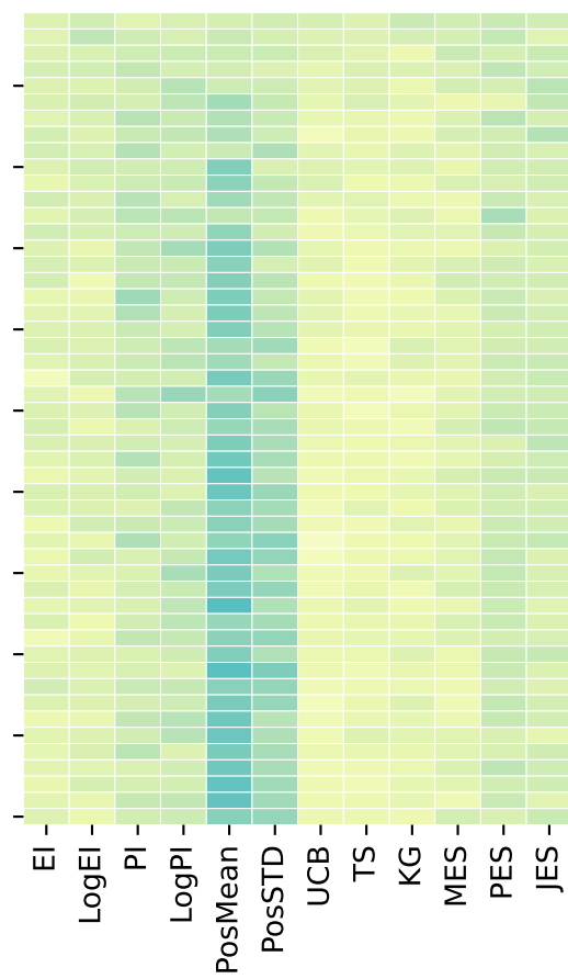
No-PASt-BO
