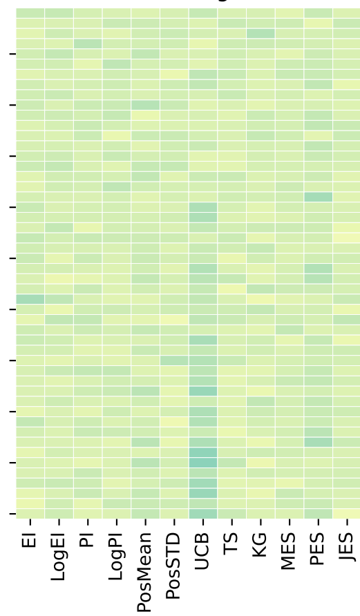
GP-Hedge
