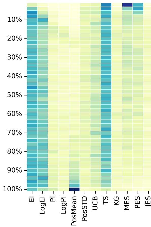
LMABO
