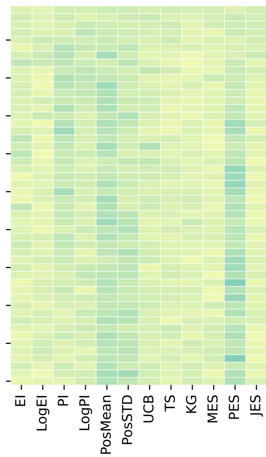
SETUP-BO
