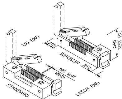
5254-050/-100 SERIES (LOW PROFILE VERSION)
