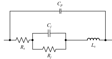
Fig. 1 SPICE model of tunnel diode
