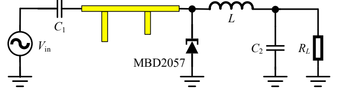
Fig. 3 Schematic of rectifier based on tunnel diode
