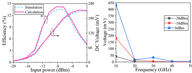
Fig. 6 (a)Simulation and calculation results of efficiency and dc voltage and (b) simulated spectrum of the rectifier when f=10 GHz
