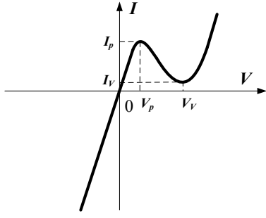
Fig. 2 I-V characteristic curve of tunnel diode
