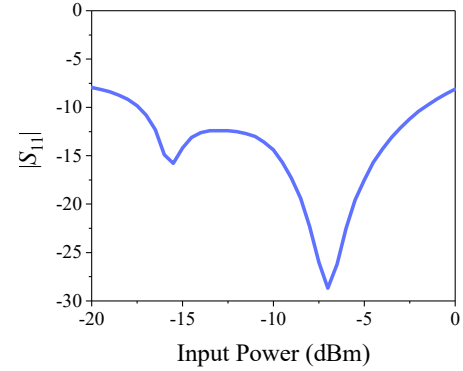
Fig. 4 |S_{11}| of the rectifier
