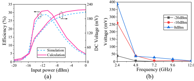
Fig. 5 (a)Simulation and calculation results of efficiency and dc voltage and (b) simulated spectrum of the rectifier when f=2.45 GHz
