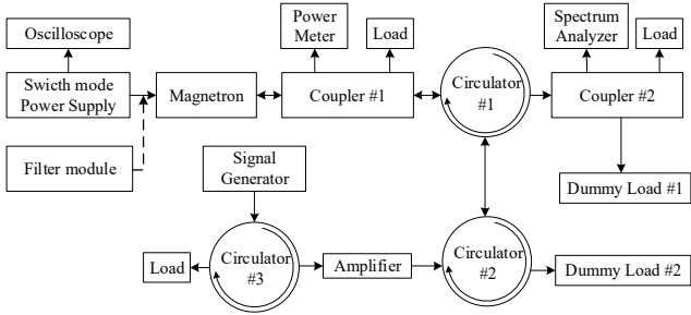
Fig. 2. Diagram of the experiment system.
