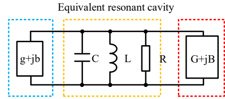
Fig. 1. Equivalent circuits of a magnetron's resonant cavity.
