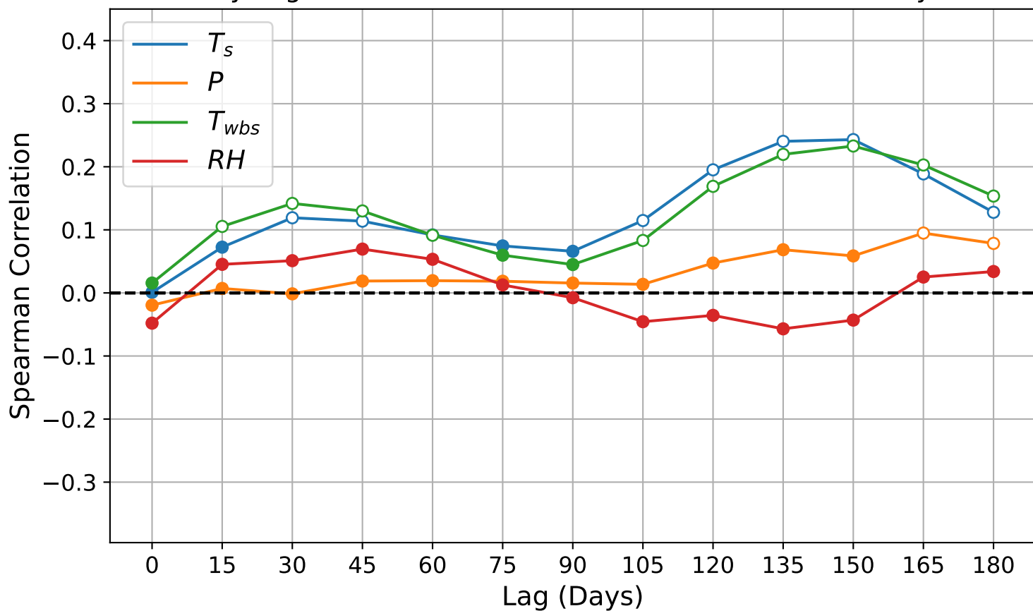
B. Daily Lag Correlations for Weather Variables vs Positivity Rate
