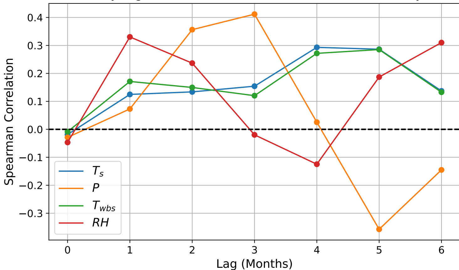
A. Monthly Lag Correlations for Weather Variables vs Positivity Rate
