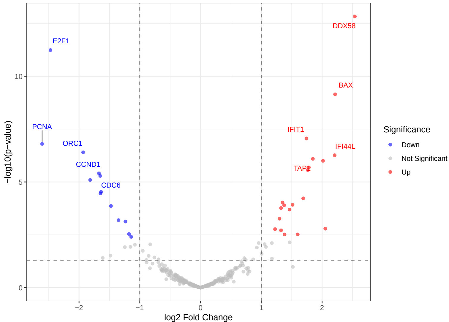
Volcano Plot: cisplatin_vs_vehicle
