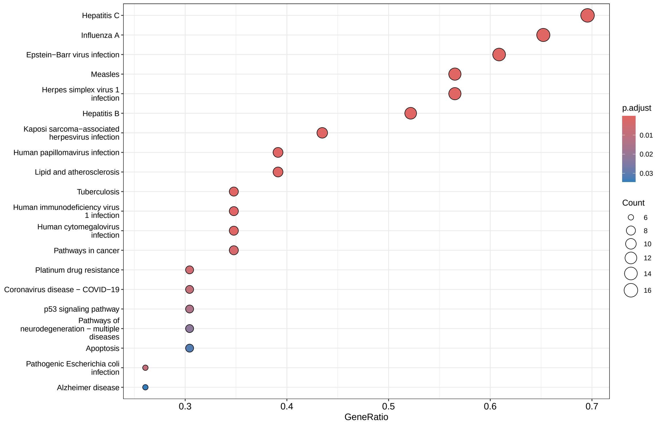
KEGG Pathways – cisplatin_vs_vehicle
