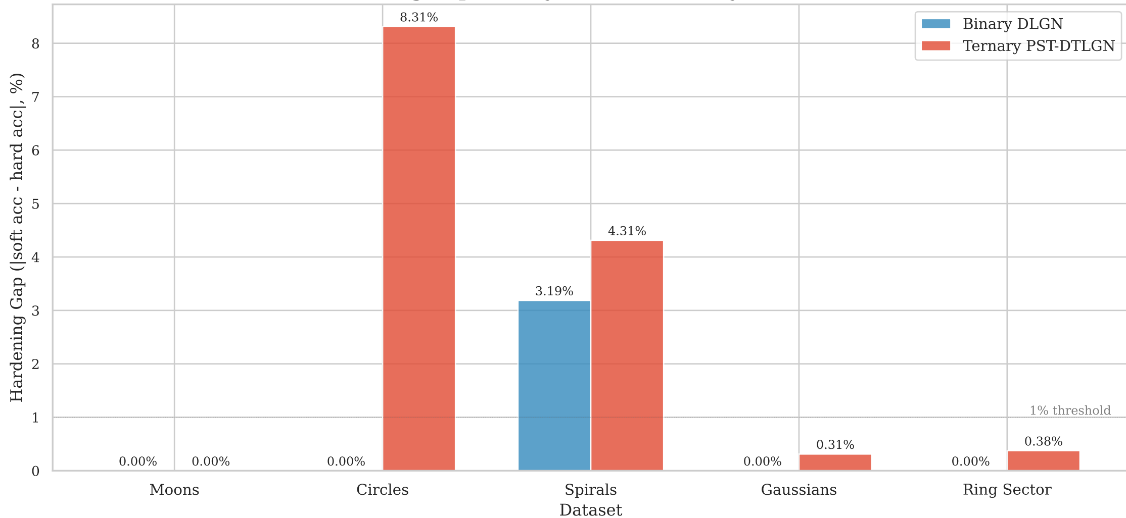
Hardening Gap: Binary DLGN vs Ternary PST-DTLGN
