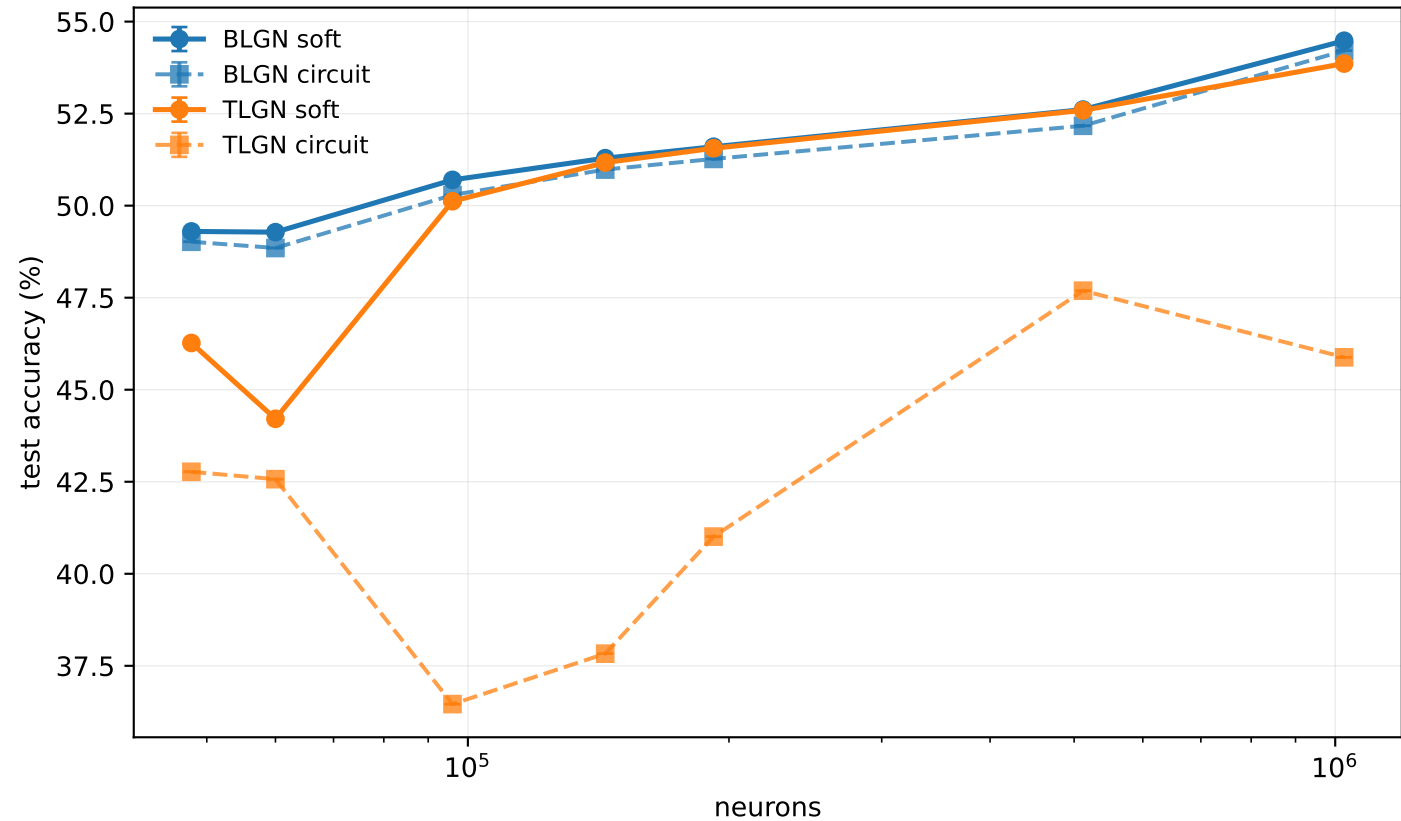
Scaling: soft network vs hardened circuit
