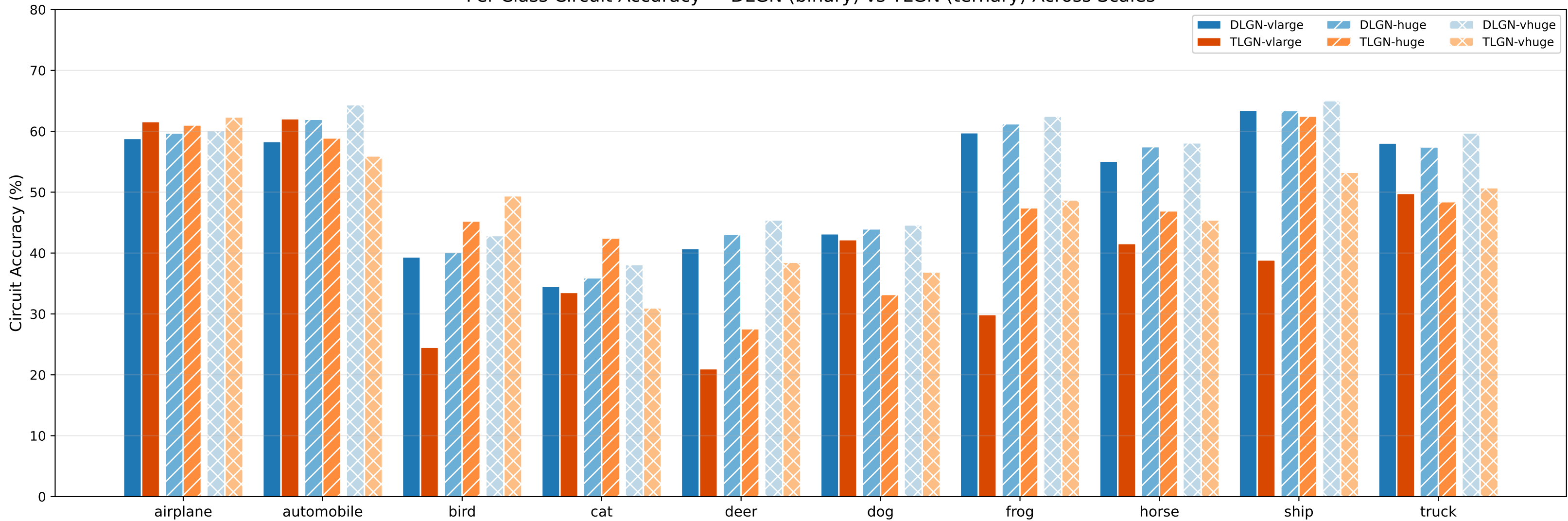
Per-Class Circuit Accuracy — DLGN (binary) vs TLGN (ternary) Across Scales
