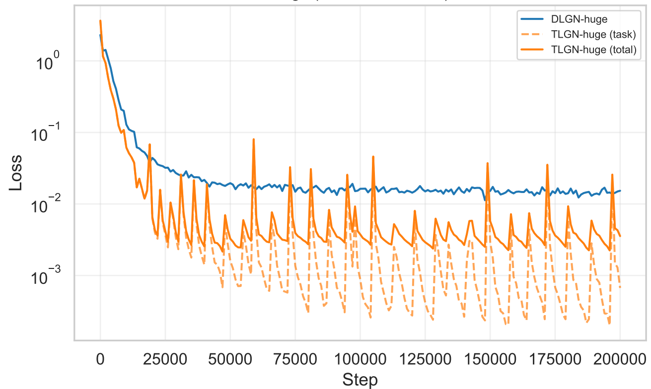
Huge (512K neurons, 4L)
